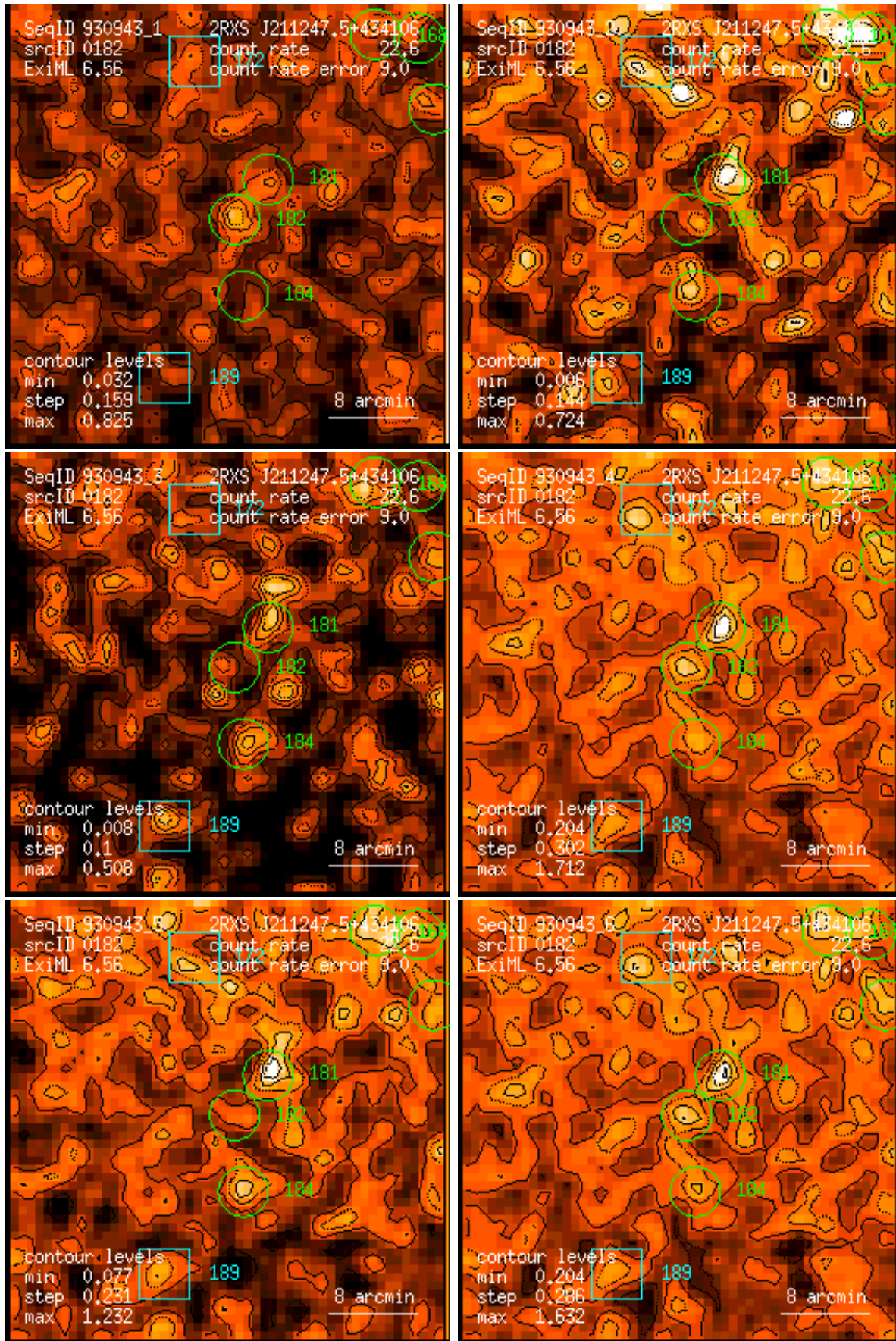
Figure 182: RASS 930943: detection 0182: band rate images, Gaussian filter: (1) PSPC channels 11 – 41, (2) 52 – 90, (3) 91 – 201, (4) 11 – 235, (5) 52 – 201, (6) 11 – 201. Broad band rates in counts/ks. Band rate contour levels in counts/ks/arcmin 2 .
