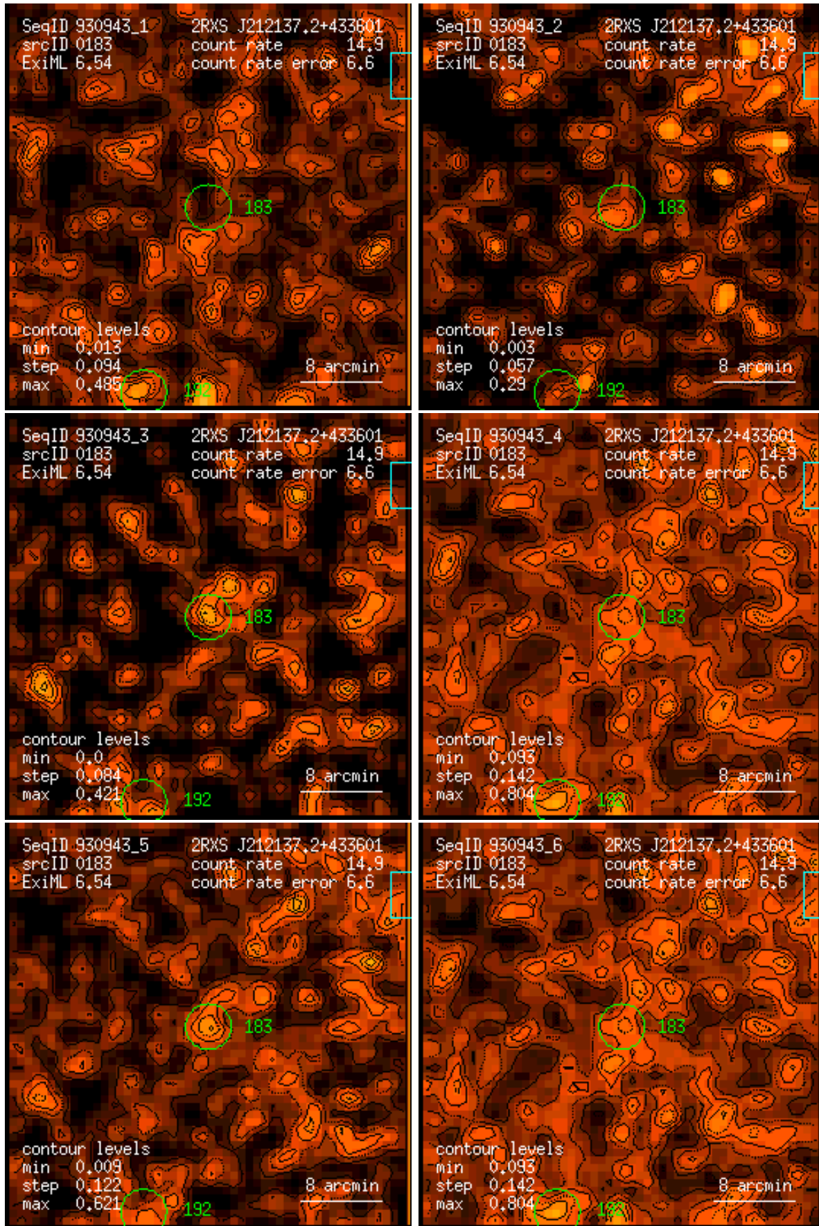
Figure 183: RASS 930943: detection 0183: band rate images, Gaussian filter: (1) PSPC channels 11 – 41, (2) 52 – 90, (3) 91 – 201, (4) 11 – 235, (5) 52 – 201, (6) 11 – 201. Broad band rates in counts/ks. Band rate contour levels in counts/ks/arcmin 2 .
