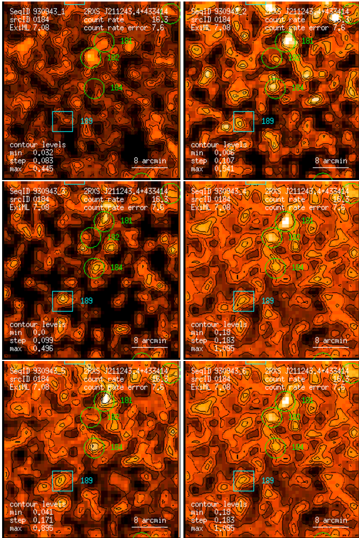
Figure 184: RASS 930943: detection 0184: band rate images, Gaussian filter: (1) PSPC channels 11 – 41, (2) 52 – 90, (3) 91 – 201, (4) 11 – 235, (5) 52 – 201, (6) 11 – 201. Broad band rates in counts/ks. Band rate contour levels in counts/ks/arcmin 2 .
