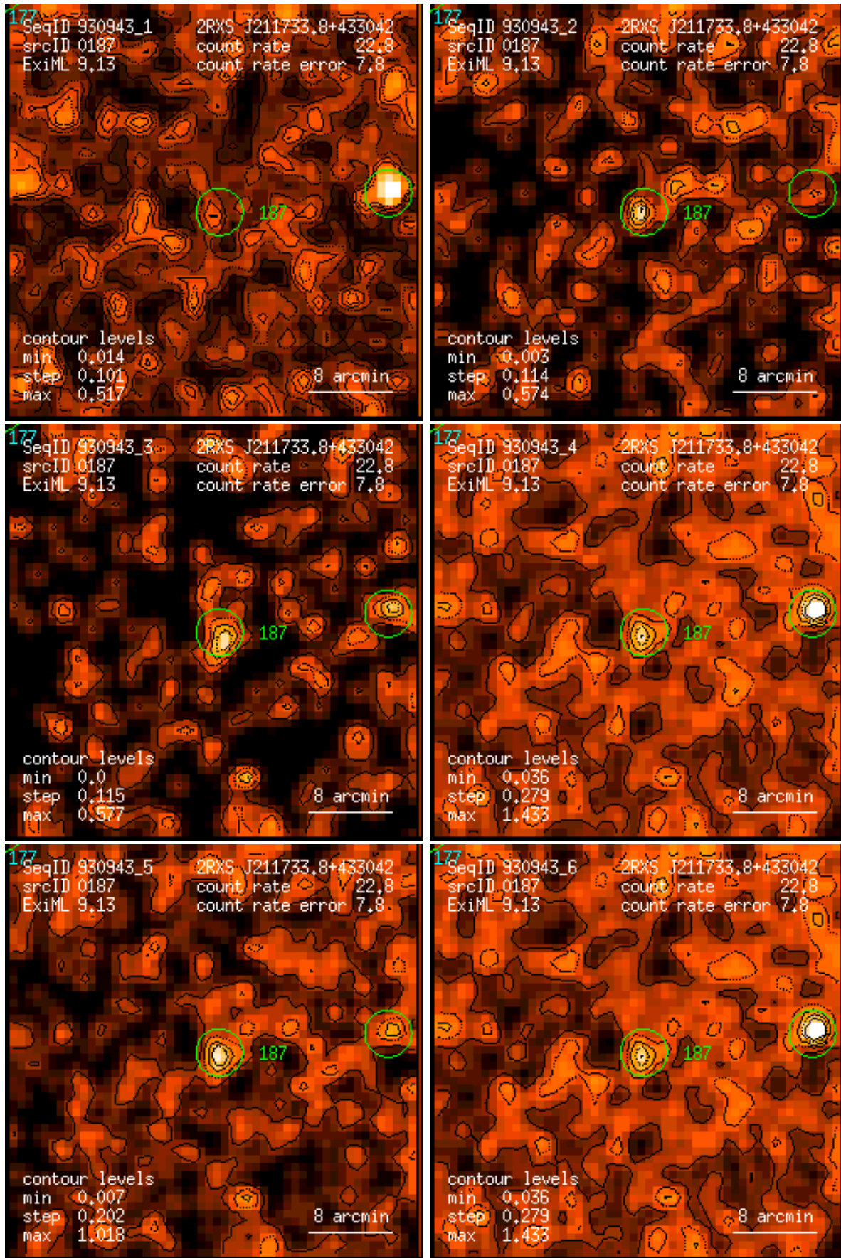
Figure 187: RASS 930943: detection 0187: band rate images, Gaussian filter: (1) PSPC channels 11 – 41, (2) 52 – 90, (3) 91 – 201, (4) 11 – 235, (5) 52 – 201, (6) 11 – 201. Broad band rates in counts/ks. Band rate contour levels in counts/ks/arcmin 2 .
