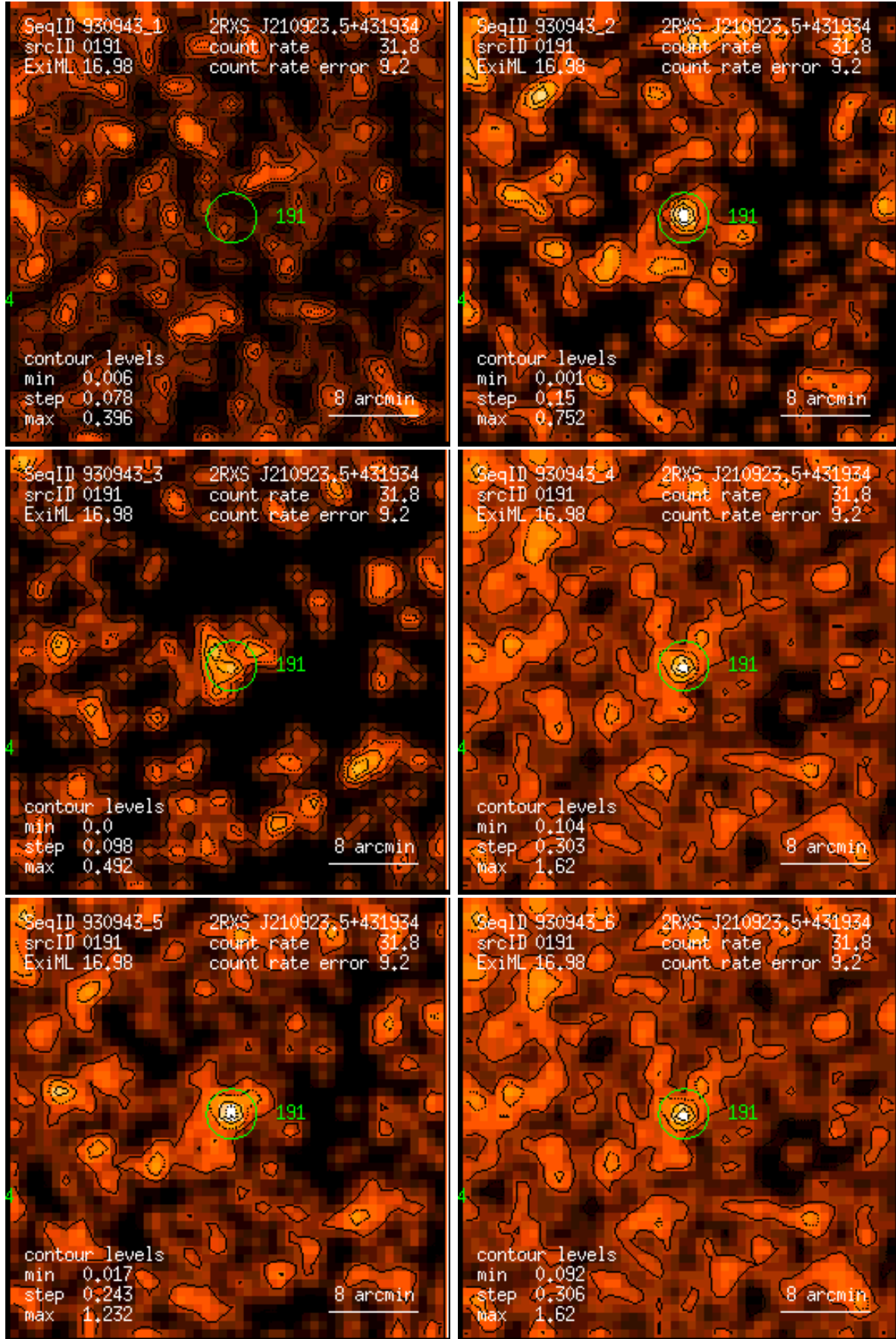
Figure 191: RASS 930943: detection 0191: band rate images, Gaussian filter: (1) PSPC channels 11 – 41, (2) 52 – 90, (3) 91 – 201, (4) 11 – 235, (5) 52 – 201, (6) 11 – 201. Broad band rates in counts/ks. Band rate contour levels in counts/ks/arcmin 2 .
