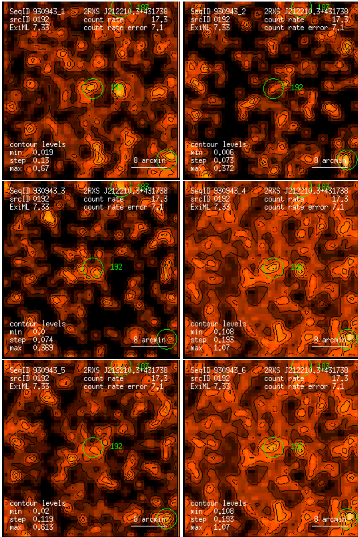
Figure 192: RASS 930943: detection 0192: band rate images, Gaussian filter: (1) PSPC channels 11 – 41, (2) 52 – 90, (3) 91 – 201, (4) 11 – 235, (5) 52 – 201, (6) 11 – 201. Broad band rates in counts/ks. Band rate contour levels in counts/ks/arcmin 2 .
