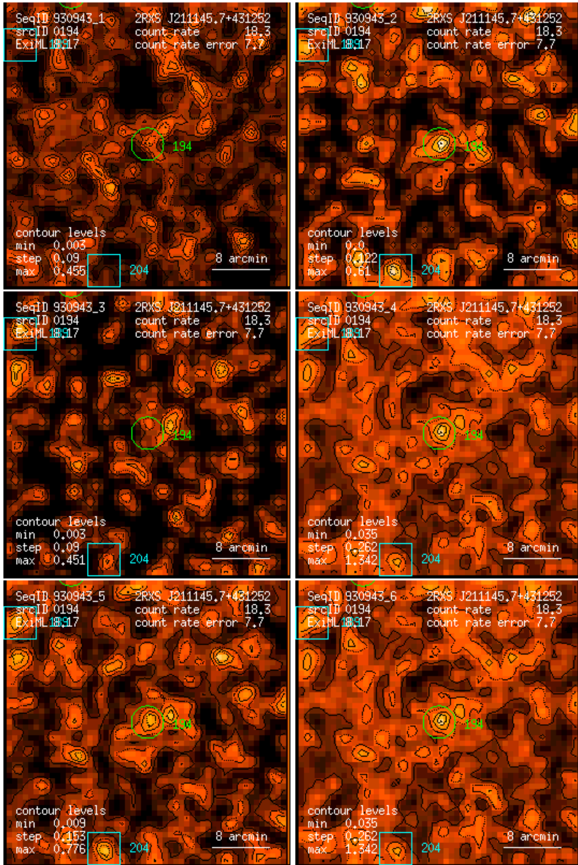
Figure 194: RASS 930943: detection 0194: band rate images, Gaussian filter: (1) PSPC channels 11 – 41, (2) 52 – 90, (3) 91 – 201, (4) 11 – 235, (5) 52 – 201, (6) 11 – 201. Broad band rates in counts/ks. Band rate contour levels in counts/ks/arcmin 2 .
