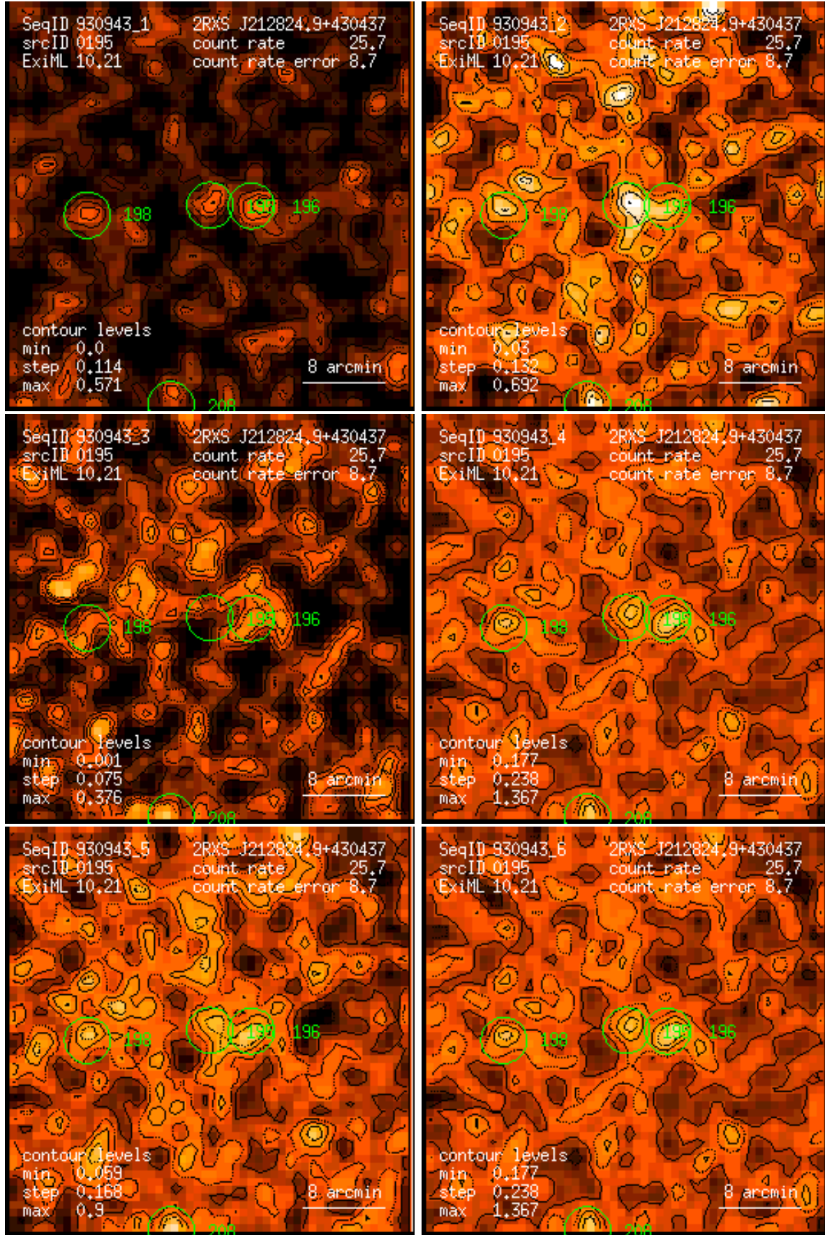
Figure 195: RASS 930943: detection 0195: band rate images, Gaussian filter: (1) PSPC channels 11 – 41, (2) 52 – 90, (3) 91 – 201, (4) 11 – 235, (5) 52 – 201, (6) 11 – 201. Broad band rates in counts/ks. Band rate contour levels in counts/ks/arcmin 2 .
