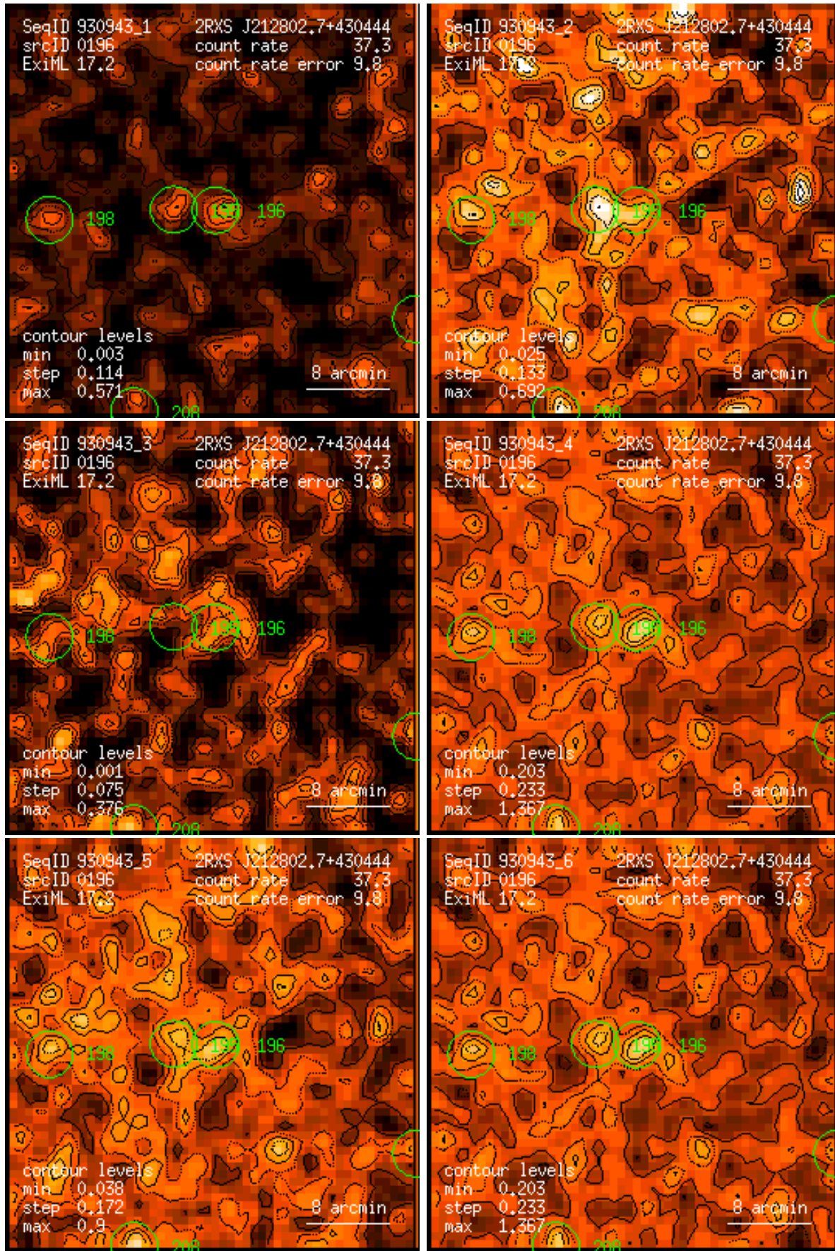
Figure 196: RASS 930943: detection 0196: band rate images, Gaussian filter: (1) PSPC channels 11 – 41, (2) 52 – 90, (3) 91 – 201, (4) 11 – 235, (5) 52 – 201, (6) 11 – 201. Broad band rates in counts/ks. Band rate contour levels in counts/ks/arcmin 2 .
