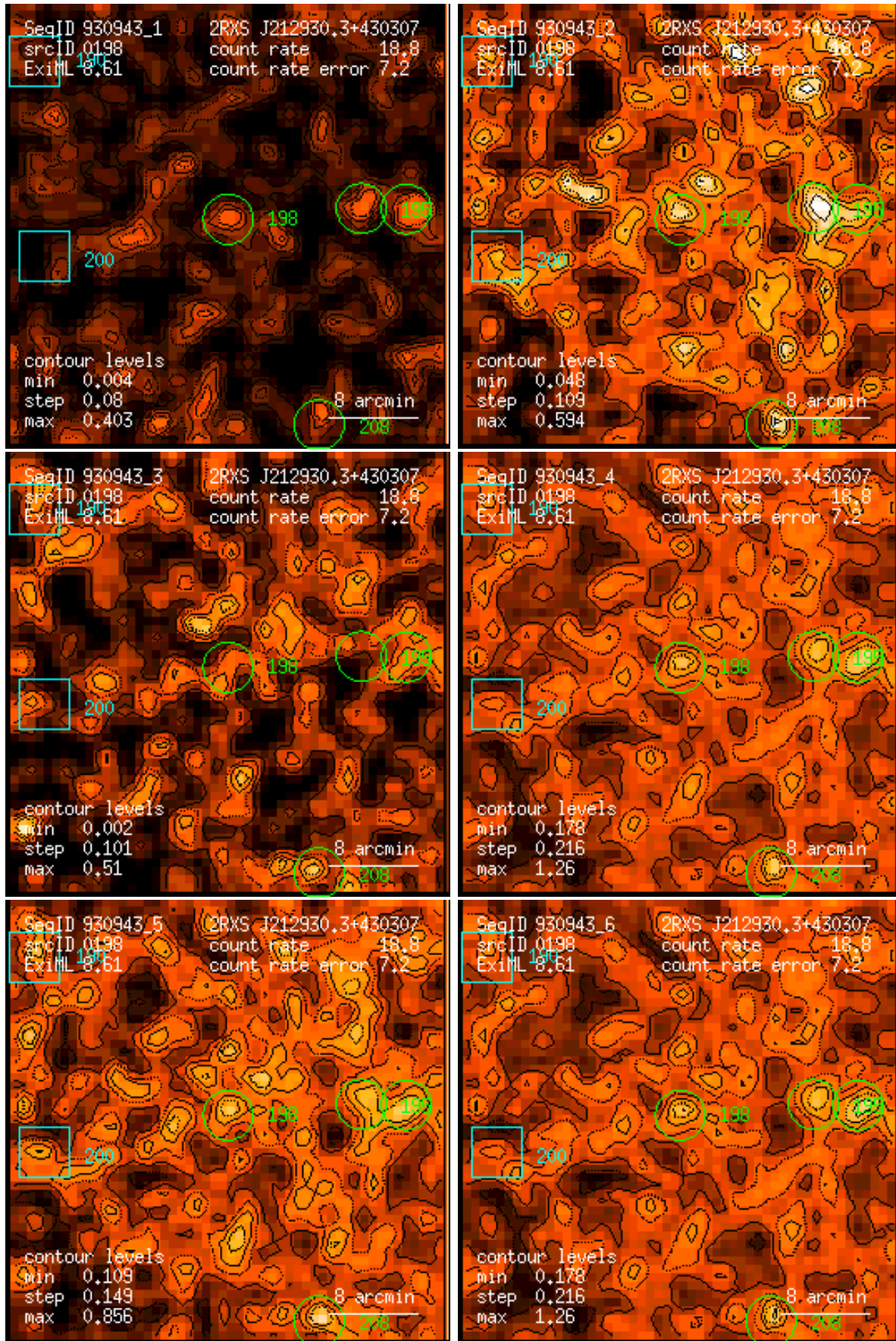
Figure 198: RASS 930943: detection 0198: band rate images, Gaussian filter: (1) PSPC channels 11 – 41, (2) 52 – 90, (3) 91 – 201, (4) 11 – 235, (5) 52 – 201, (6) 11 – 201. Broad band rates in counts/ks. Band rate contour levels in counts/ks/arcmin 2 .
