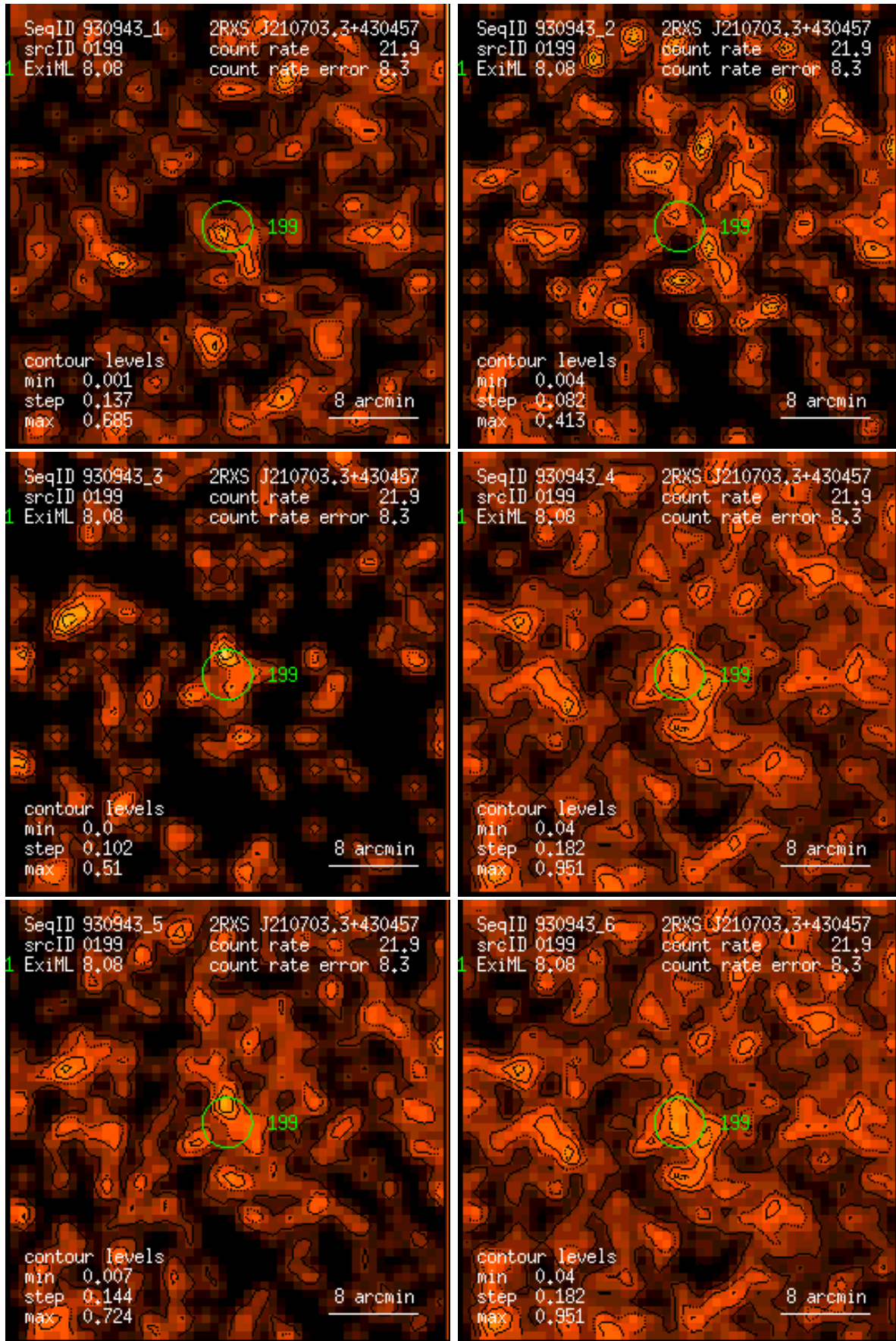
Figure 199: RASS 930943: detection 0199: band rate images, Gaussian filter: (1) PSPC channels 11 – 41, (2) 52 – 90, (3) 91 – 201, (4) 11 – 235, (5) 52 – 201, (6) 11 – 201. Broad band rates in counts/ks. Band rate contour levels in counts/ks/arcmin 2 .
