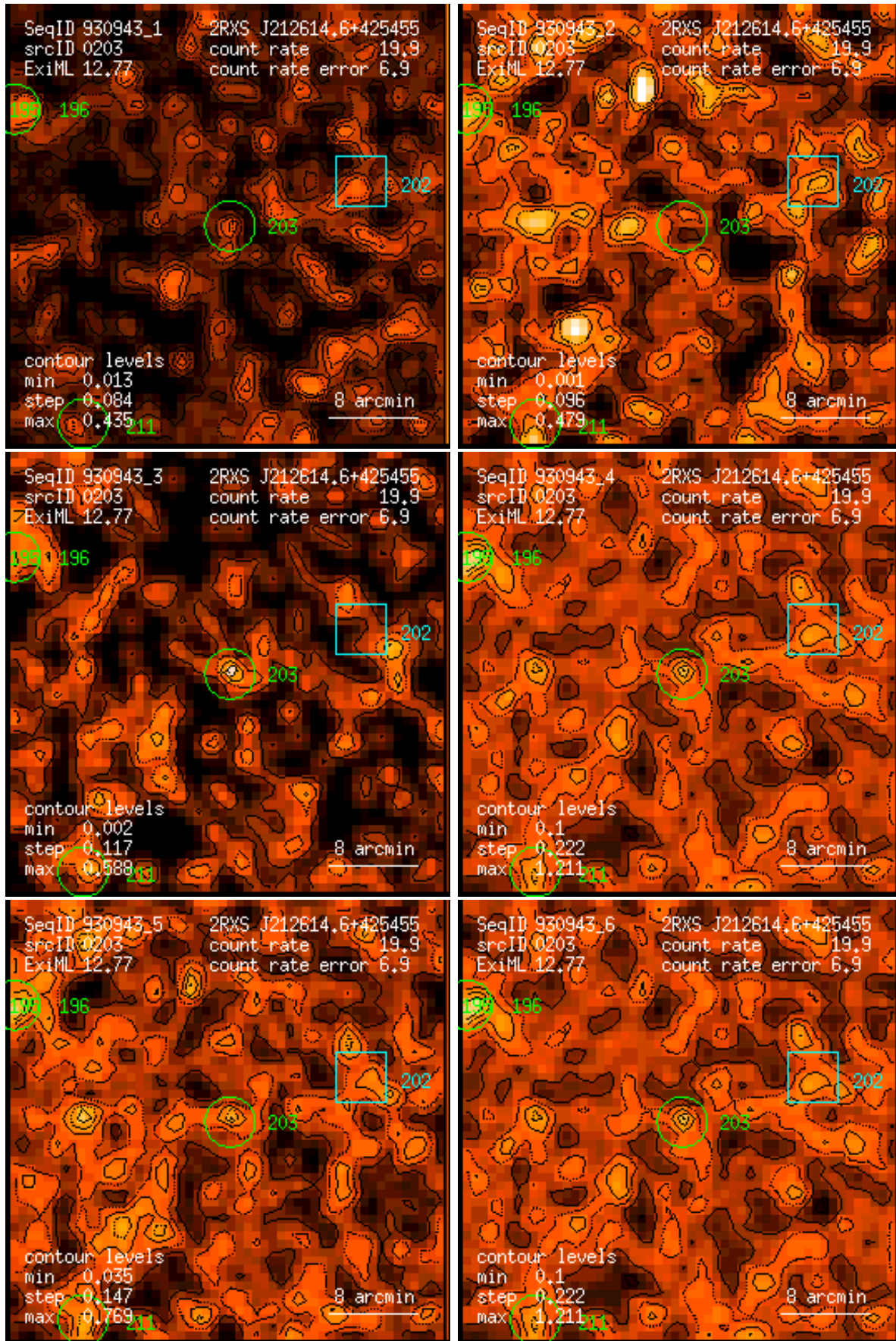
Figure 203: RASS 930943: detection 0203: band rate images, Gaussian filter: (1) PSPC channels 11 – 41, (2) 52 – 90, (3) 91 – 201, (4) 11 – 235, (5) 52 – 201, (6) 11 – 201. Broad band rates in counts/ks. Band rate contour levels in counts/ks/arcmin 2 .
