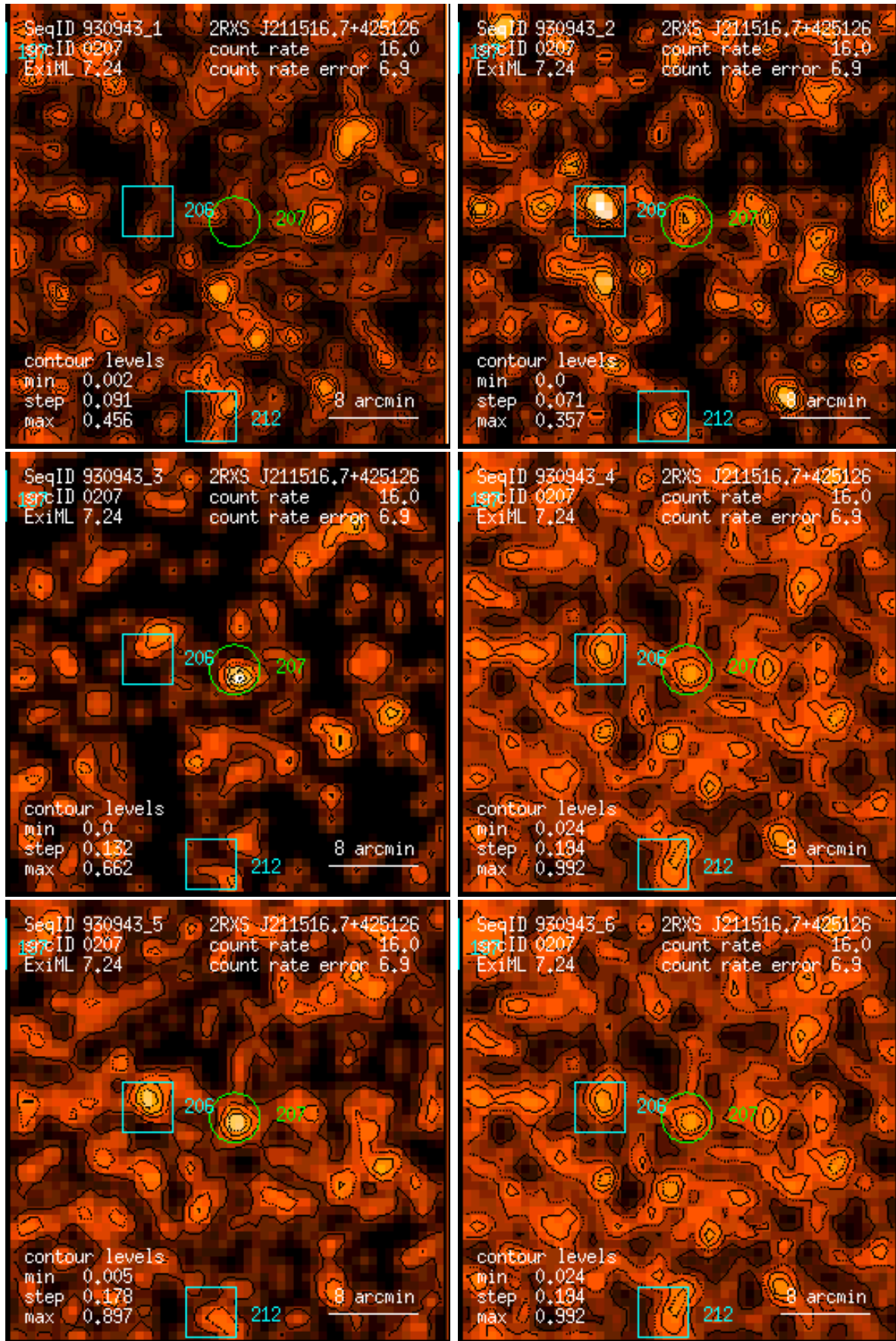
Figure 207: RASS 930943: detection 0207: band rate images, Gaussian filter: (1) PSPC channels 11 – 41, (2) 52 – 90, (3) 91 – 201, (4) 11 – 235, (5) 52 – 201, (6) 11 – 201. Broad band rates in counts/ks. Band rate contour levels in counts/ks/arcmin 2 .
