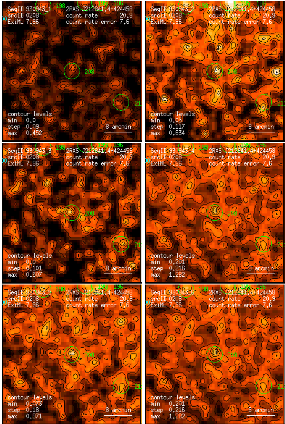
Figure 208: RASS 930943: detection 0208: band rate images, Gaussian filter: (1) PSPC channels 11 – 41, (2) 52 – 90, (3) 91 – 201, (4) 11 – 235, (5) 52 – 201, (6) 11 – 201. Broad band rates in counts/ks. Band rate contour levels in counts/ks/arcmin 2 .
