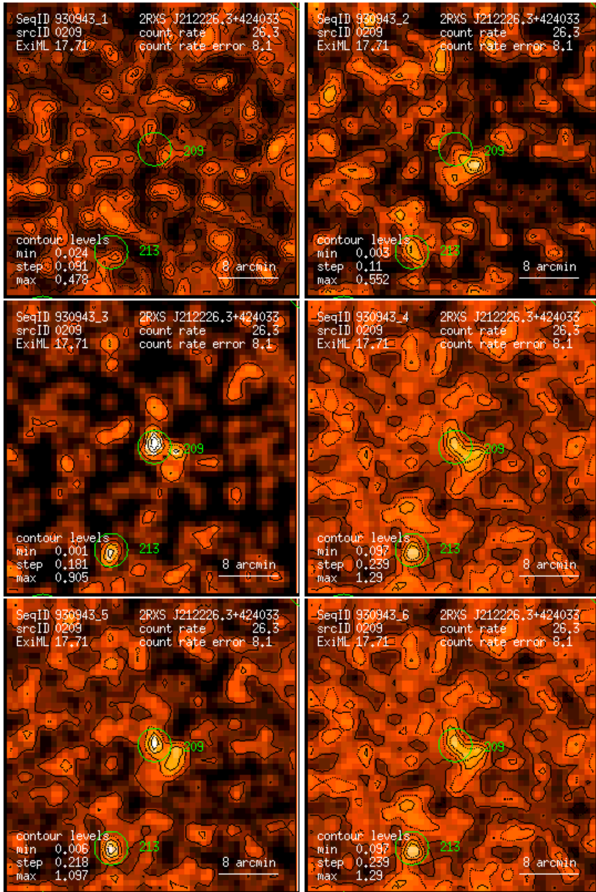
Figure 209: RASS 930943: detection 0209: band rate images, Gaussian filter: (1) PSPC channels 11 – 41, (2) 52 – 90, (3) 91 – 201, (4) 11 – 235, (5) 52 – 201, (6) 11 – 201. Broad band rates in counts/ks. Band rate contour levels in counts/ks/arcmin 2 .
