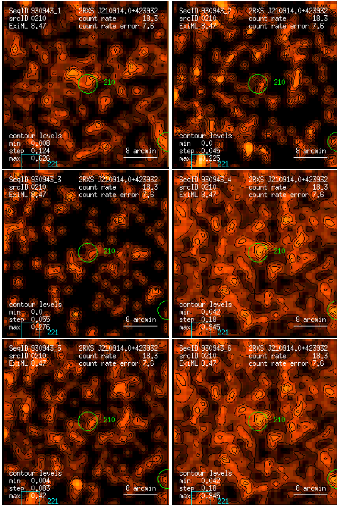
Figure 210: RASS 930943: detection 0210: band rate images, Gaussian filter: (1) PSPC channels 11 – 41, (2) 52 – 90, (3) 91 – 201, (4) 11 – 235, (5) 52 – 201, (6) 11 – 201. Broad band rates in counts/ks. Band rate contour levels in counts/ks/arcmin 2 .
