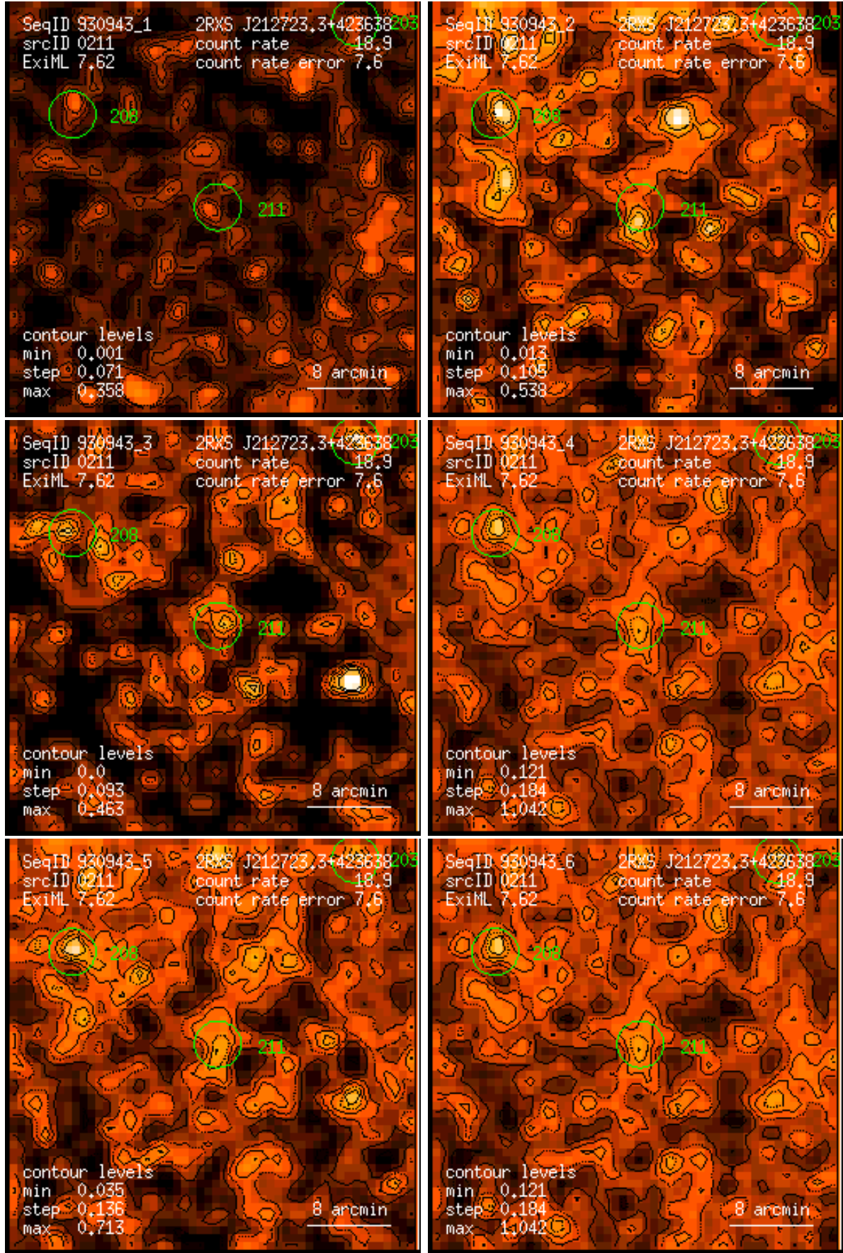
Figure 211: RASS 930943: detection 0211: band rate images, Gaussian filter: (1) PSPC channels 11 – 41, (2) 52 – 90, (3) 91 – 201, (4) 11 – 235, (5) 52 – 201, (6) 11 – 201. Broad band rates in counts/ks. Band rate contour levels in counts/ks/arcmin 2 .
