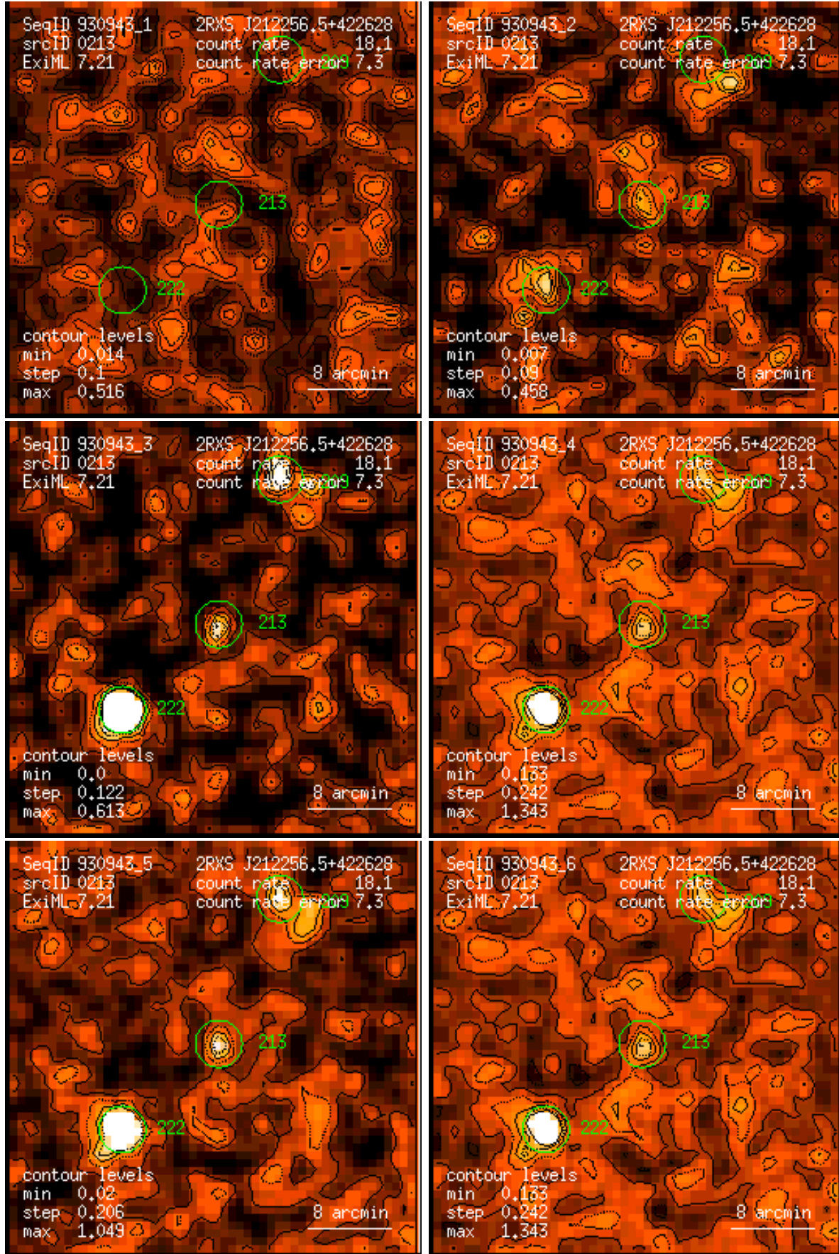
Figure 213: RASS 930943: detection 0213: band rate images, Gaussian filter: (1) PSPC channels 11 – 41, (2) 52 – 90, (3) 91 – 201, (4) 11 – 235, (5) 52 – 201, (6) 11 – 201. Broad band rates in counts/ks. Band rate contour levels in counts/ks/arcmin 2 .
