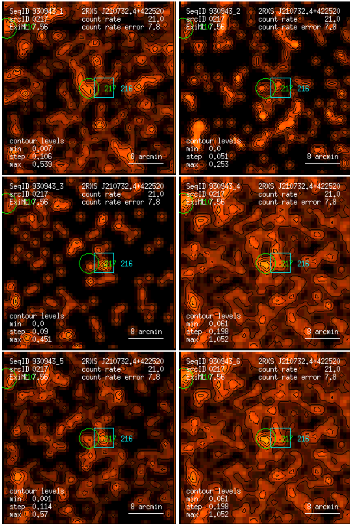
Figure 217: RASS 930943: detection 0217: band rate images, Gaussian filter: (1) PSPC channels 11 – 41, (2) 52 – 90, (3) 91 – 201, (4) 11 – 235, (5) 52 – 201, (6) 11 – 201. Broad band rates in counts/ks. Band rate contour levels in counts/ks/arcmin 2 .
