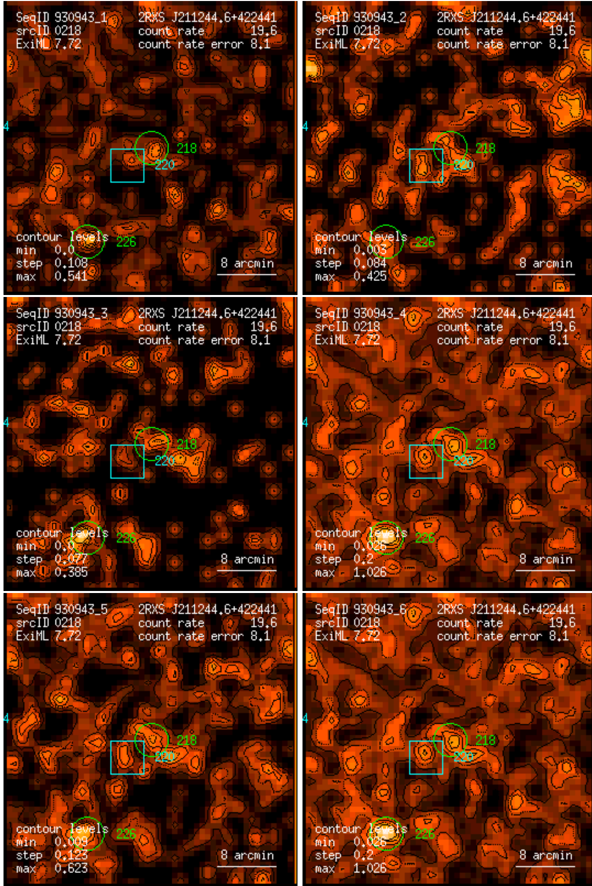
Figure 218: RASS 930943: detection 0218: band rate images, Gaussian filter: (1) PSPC channels 11 – 41, (2) 52 – 90, (3) 91 – 201, (4) 11 – 235, (5) 52 – 201, (6) 11 – 201. Broad band rates in counts/ks. Band rate contour levels in counts/ks/arcmin 2 .
