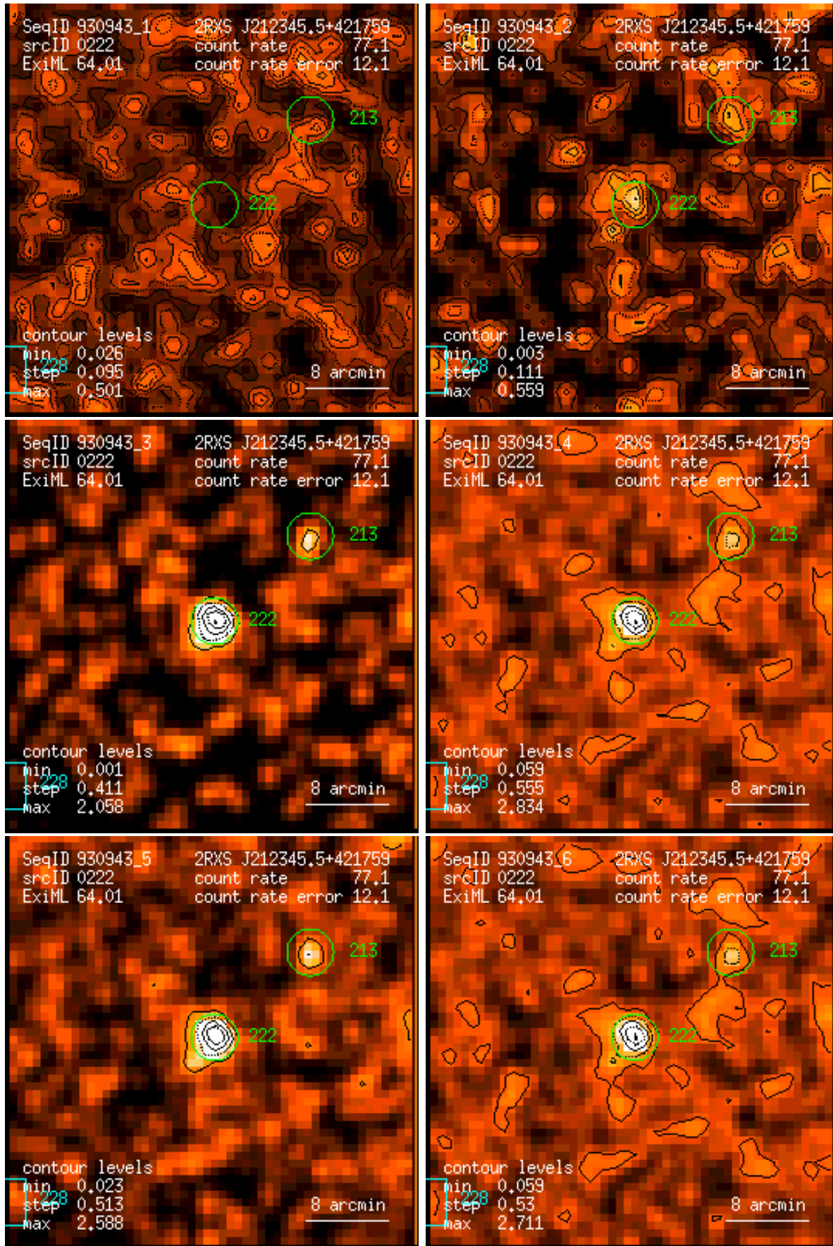
Figure 222: RASS 930943: detection 0222: band rate images, Gaussian filter: (1) PSPC channels 11 – 41, (2) 52 – 90, (3) 91 – 201, (4) 11 – 235, (5) 52 – 201, (6) 11 – 201. Broad band rates in counts/ks. Band rate contour levels in counts/ks/arcmin 2 .
