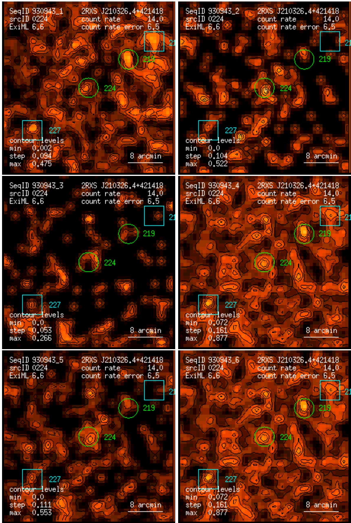
Figure 224: RASS 930943: detection 0224: band rate images, Gaussian filter: (1) PSPC channels 11 – 41, (2) 52 – 90, (3) 91 – 201, (4) 11 – 235, (5) 52 – 201, (6) 11 – 201. Broad band rates in counts/ks. Band rate contour levels in counts/ks/arcmin 2 .
