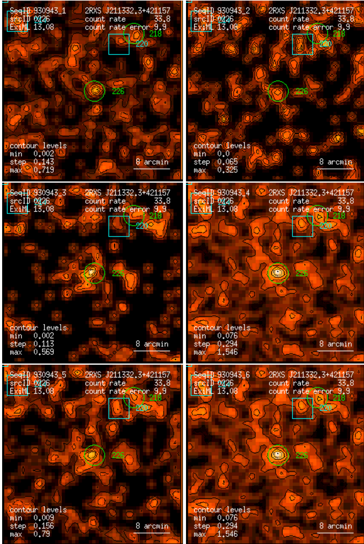
Figure 226: RASS 930943: detection 0226: band rate images, Gaussian filter: (1) PSPC channels 11 – 41, (2) 52 – 90, (3) 91 – 201, (4) 11 – 235, (5) 52 – 201, (6) 11 – 201. Broad band rates in counts/ks. Band rate contour levels in counts/ks/arcmin 2 .
