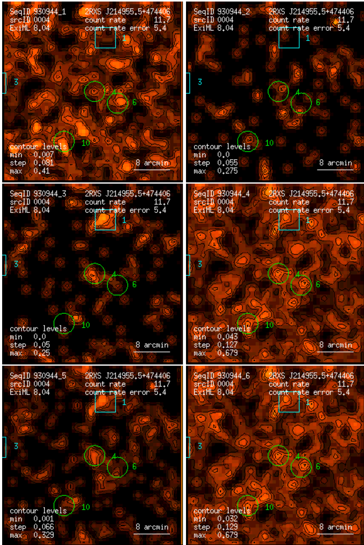
Figure 4: RASS 930944: detection 0004: band rate images, Gaussian filter: (1) PSPC channels 11 – 41, (2) 52 – 90, (3) 91 – 201, (4) 11 – 235, (5) 52 – 201, (6) 11 – 201. Broad band rates in counts/ks. Band rate contour levels in counts/ks/arcmin 2 .
