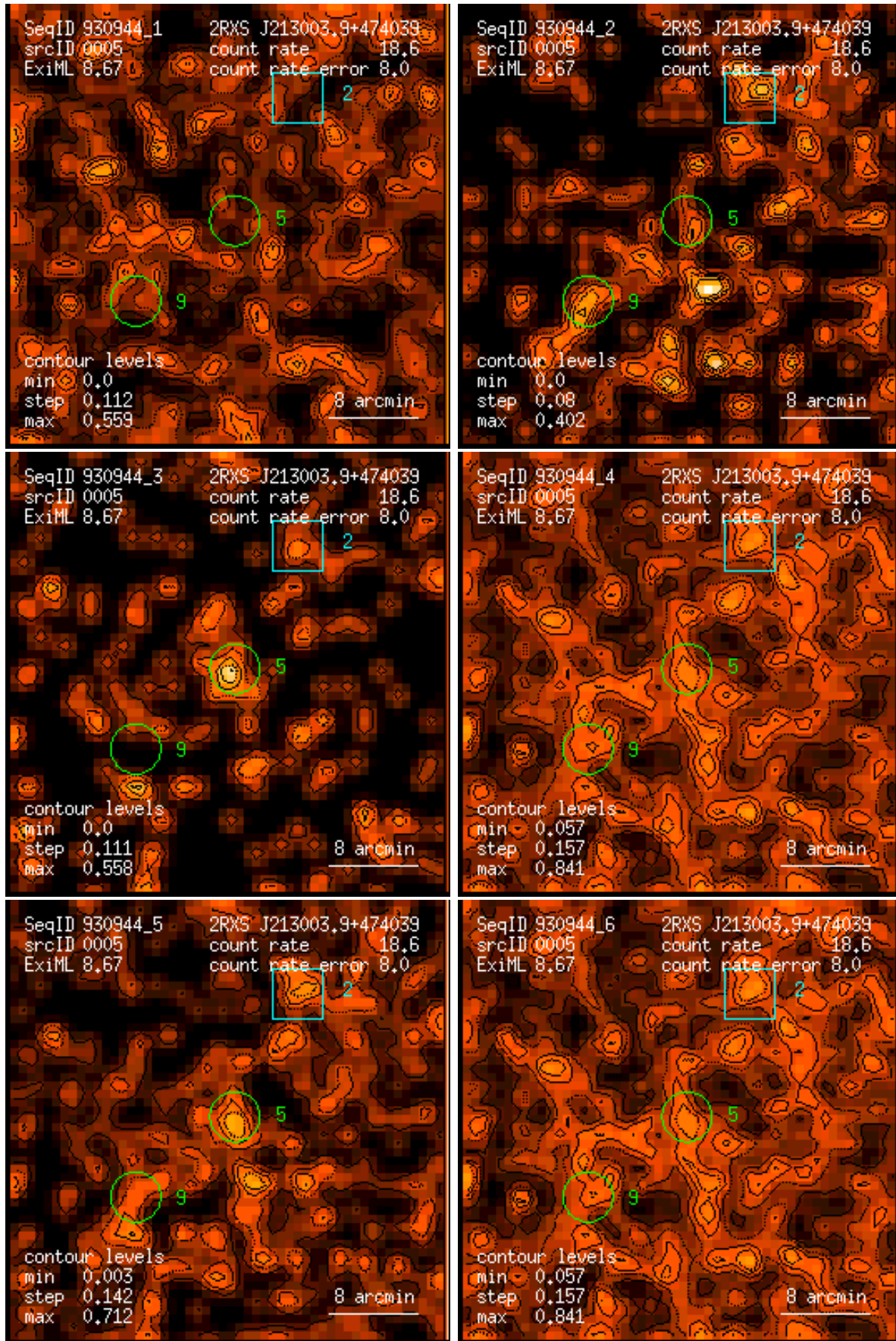
Figure 5: RASS 930944: detection 0005: band rate images, Gaussian filter: (1) PSPC channels 11 – 41, (2) 52 – 90, (3) 91 – 201, (4) 11 – 235, (5) 52 – 201, (6) 11 – 201. Broad band rates in counts/ks. Band rate contour levels in counts/ks/arcmin 2 .
