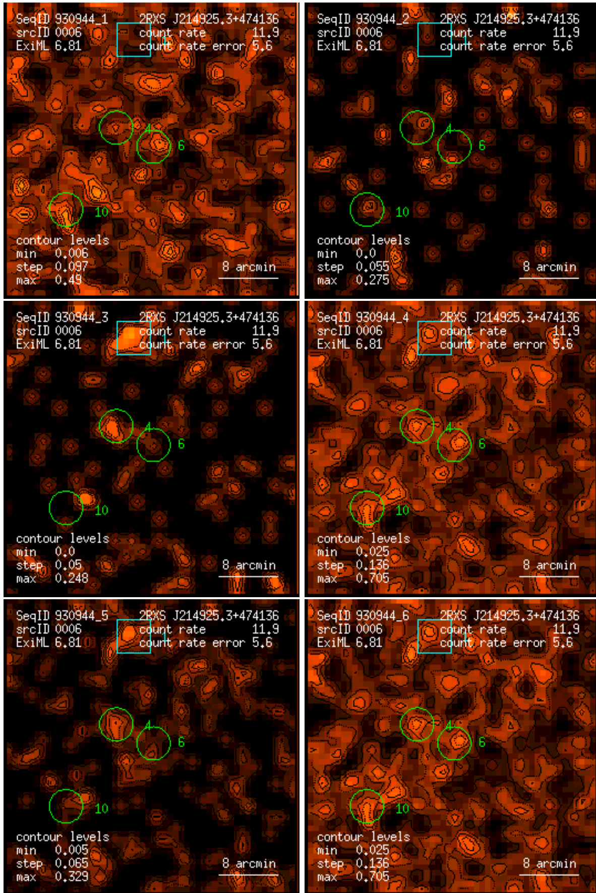
Figure 6: RASS 930944: detection 0006: band rate images, Gaussian filter: (1) PSPC channels 11 – 41, (2) 52 – 90, (3) 91 – 201, (4) 11 – 235, (5) 52 – 201, (6) 11 – 201. Broad band rates in counts/ks. Band rate contour levels in counts/ks/arcmin 2 .
