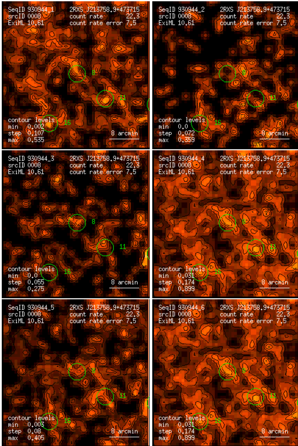
Figure 8: RASS 930944: detection 0008: band rate images, Gaussian filter: (1) PSPC channels 11 – 41, (2) 52 – 90, (3) 91 – 201, (4) 11 – 235, (5) 52 – 201, (6) 11 – 201. Broad band rates in counts/ks. Band rate contour levels in counts/ks/arcmin 2 .
