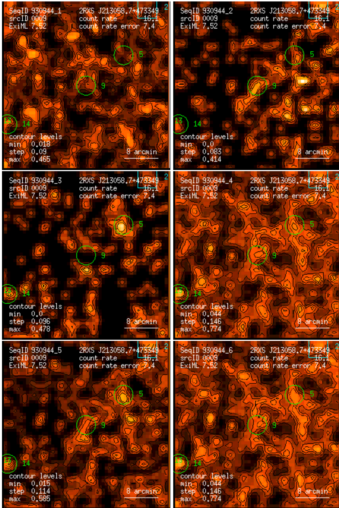
Figure 9: RASS 930944: detection 0009: band rate images, Gaussian filter: (1) PSPC channels 11 – 41, (2) 52 – 90, (3) 91 – 201, (4) 11 – 235, (5) 52 – 201, (6) 11 – 201. Broad band rates in counts/ks. Band rate contour levels in counts/ks/arcmin 2 .
