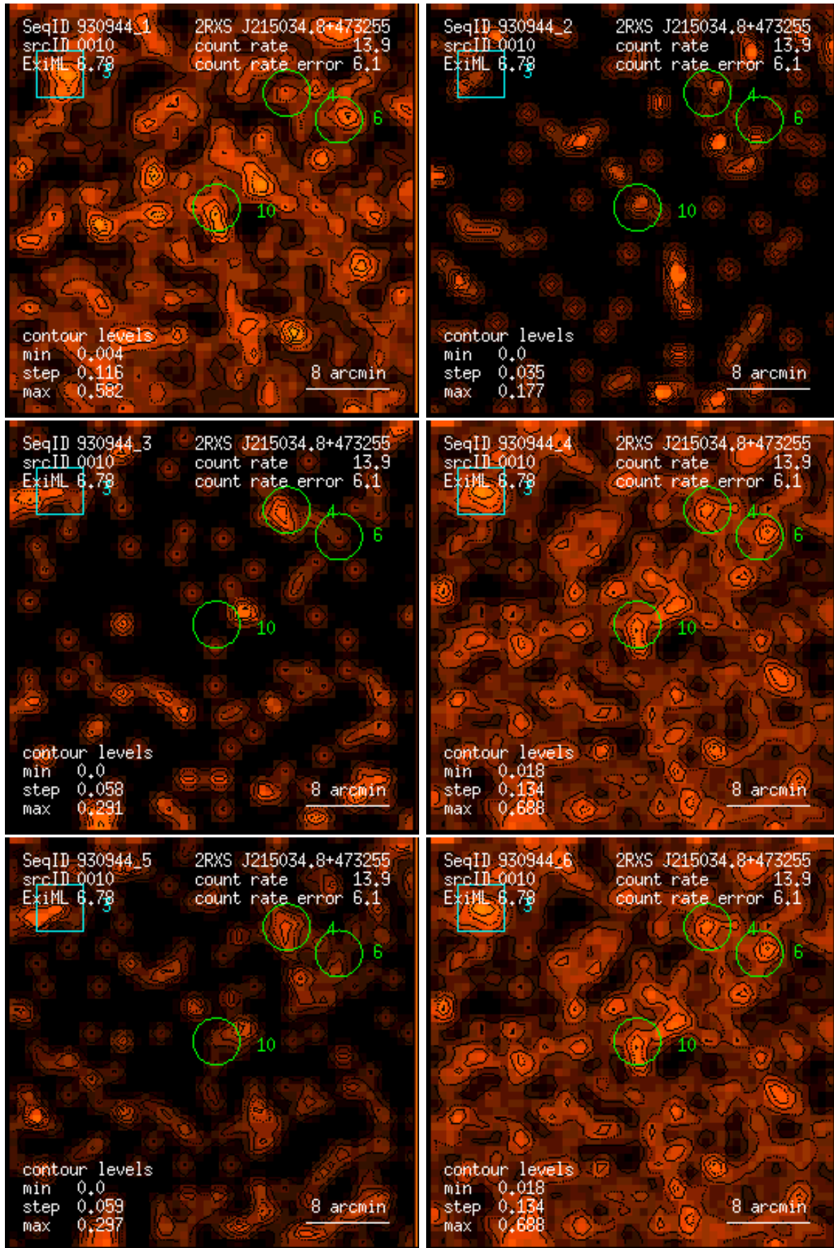
Figure 10: RASS 930944: detection 0010: band rate images, Gaussian filter: (1) PSPC channels 11 – 41, (2) 52 – 90, (3) 91 – 201, (4) 11 – 235, (5) 52 – 201, (6) 11 – 201. Broad band rates in counts/ks. Band rate contour levels in counts/ks/arcmin 2 .
