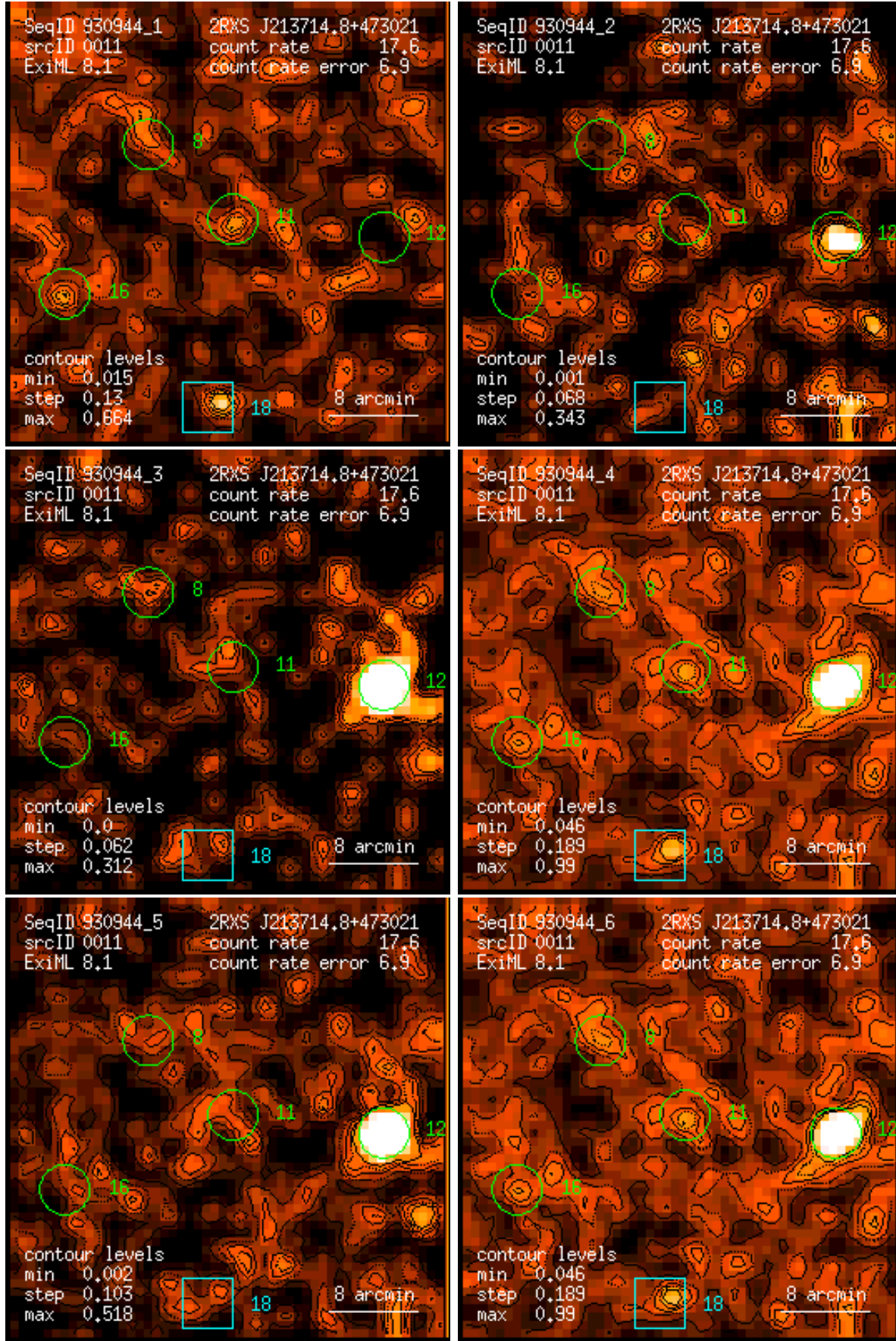
Figure 11: RASS 930944: detection 0011: band rate images, Gaussian filter: (1) PSPC channels 11 – 41, (2) 52 – 90, (3) 91 – 201, (4) 11 – 235, (5) 52 – 201, (6) 11 – 201. Broad band rates in counts/ks. Band rate contour levels in counts/ks/arcmin 2 .
