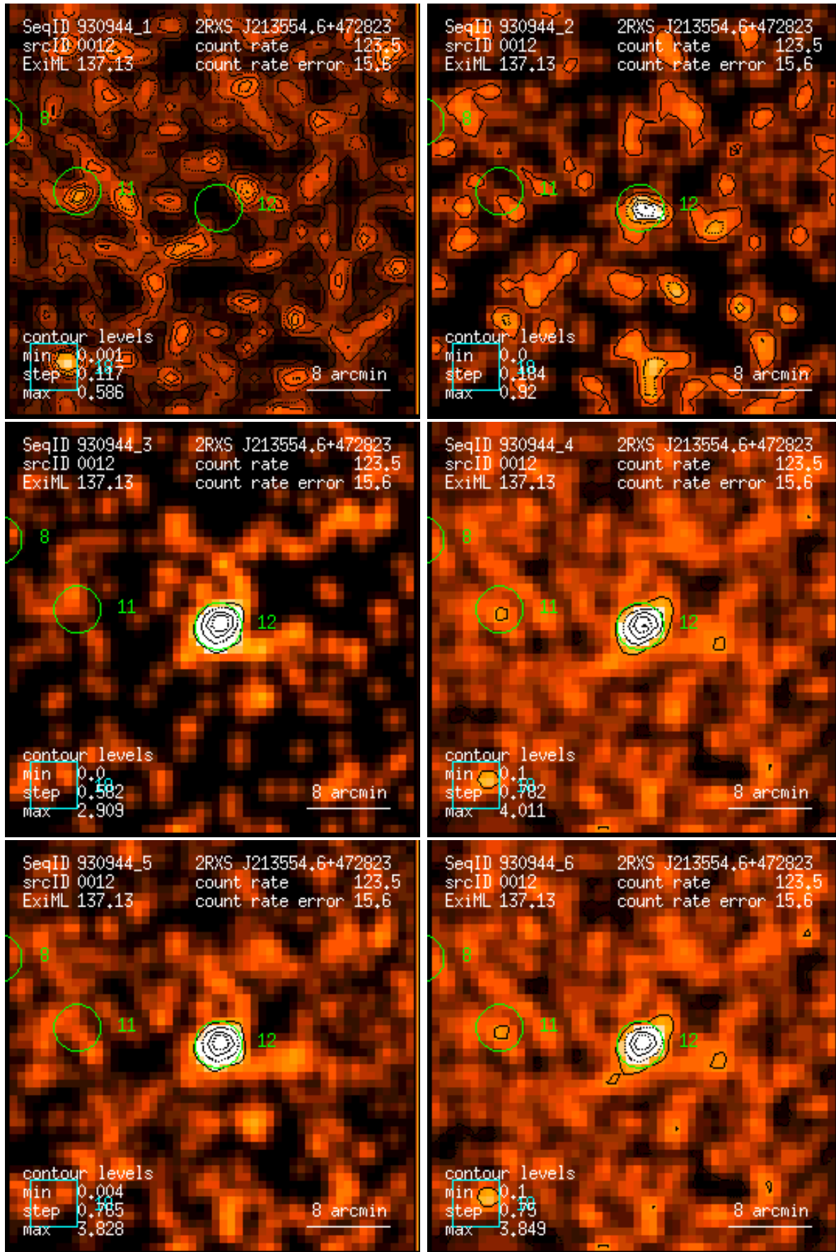
Figure 12: RASS 930944: detection 0012: band rate images, Gaussian filter: (1) PSPC channels 11 – 41, (2) 52 – 90, (3) 91 – 201, (4) 11 – 235, (5) 52 – 201, (6) 11 – 201. Broad band rates in counts/ks. Band rate contour levels in counts/ks/arcmin 2 .
