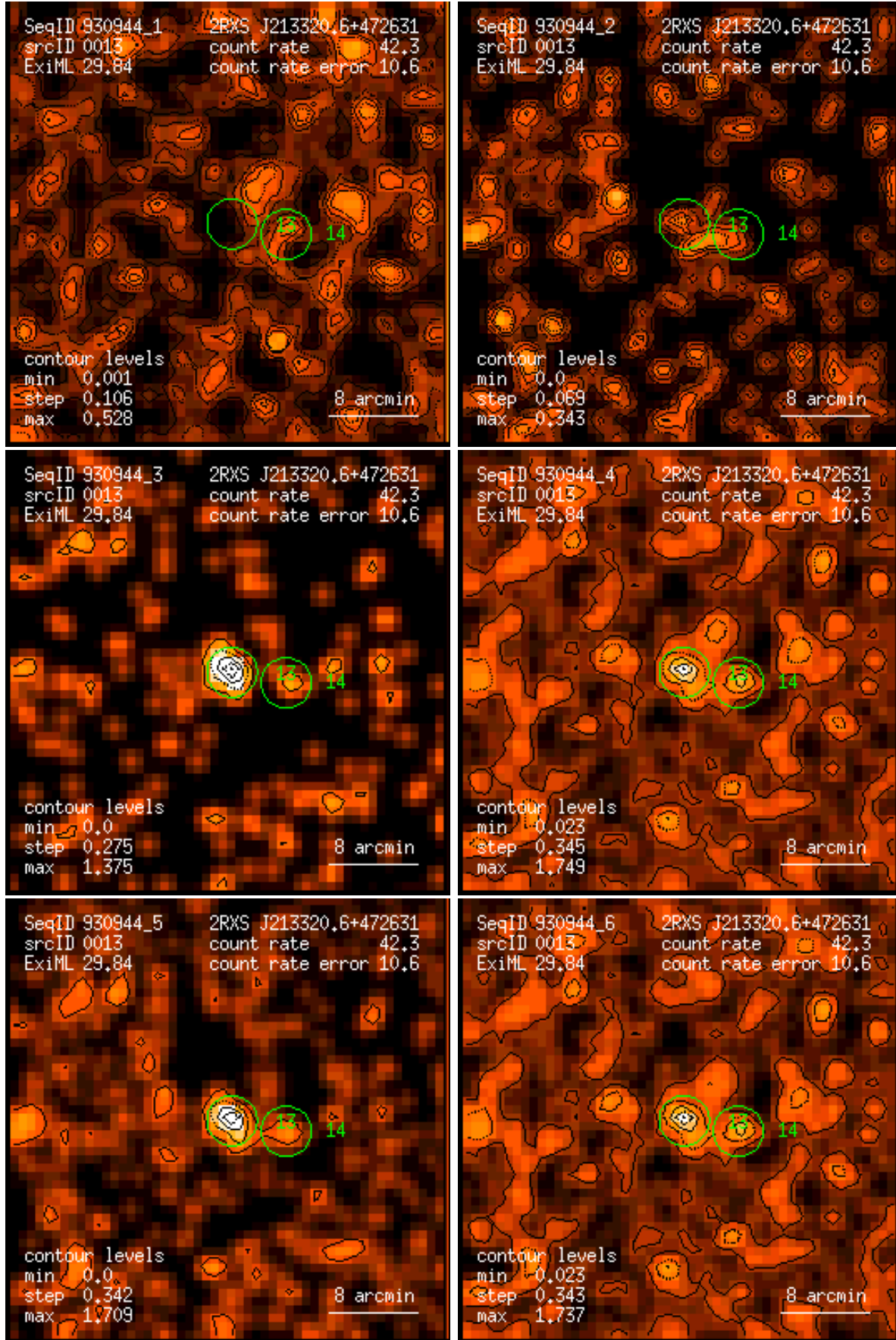
Figure 13: RASS 930944: detection 0013: band rate images, Gaussian filter: (1) PSPC channels 11 – 41, (2) 52 – 90, (3) 91 – 201, (4) 11 – 235, (5) 52 – 201, (6) 11 – 201. Broad band rates in counts/ks. Band rate contour levels in counts/ks/arcmin 2 .
