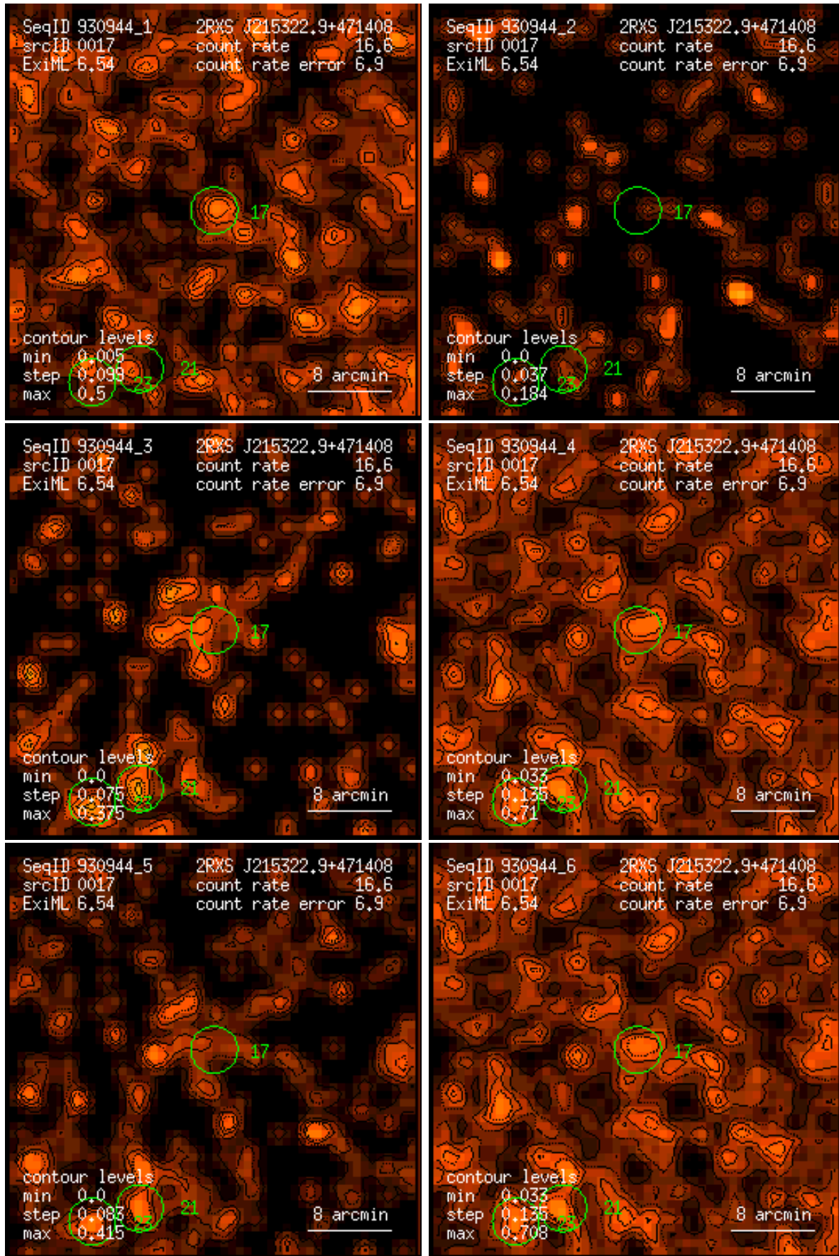
Figure 17: RASS 930944: detection 0017: band rate images, Gaussian filter: (1) PSPC channels 11 – 41, (2) 52 – 90, (3) 91 – 201, (4) 11 – 235, (5) 52 – 201, (6) 11 – 201. Broad band rates in counts/ks. Band rate contour levels in counts/ks/arcmin 2 .
