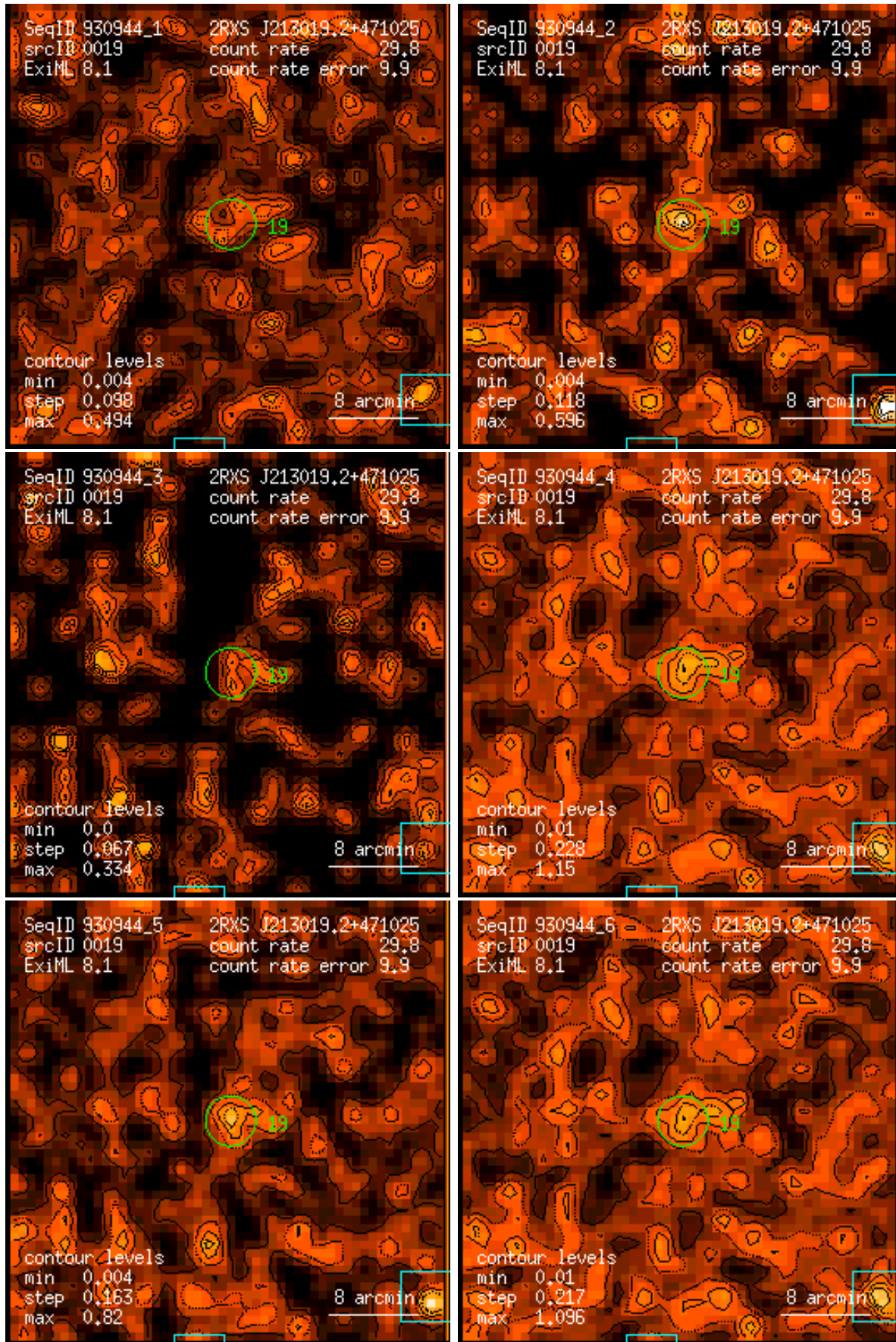
Figure 19: RASS 930944: detection 0019: band rate images, Gaussian filter: (1) PSPC channels 11 – 41, (2) 52 – 90, (3) 91 – 201, (4) 11 – 235, (5) 52 – 201, (6) 11 – 201. Broad band rates in counts/ks. Band rate contour levels in counts/ks/arcmin 2 .
