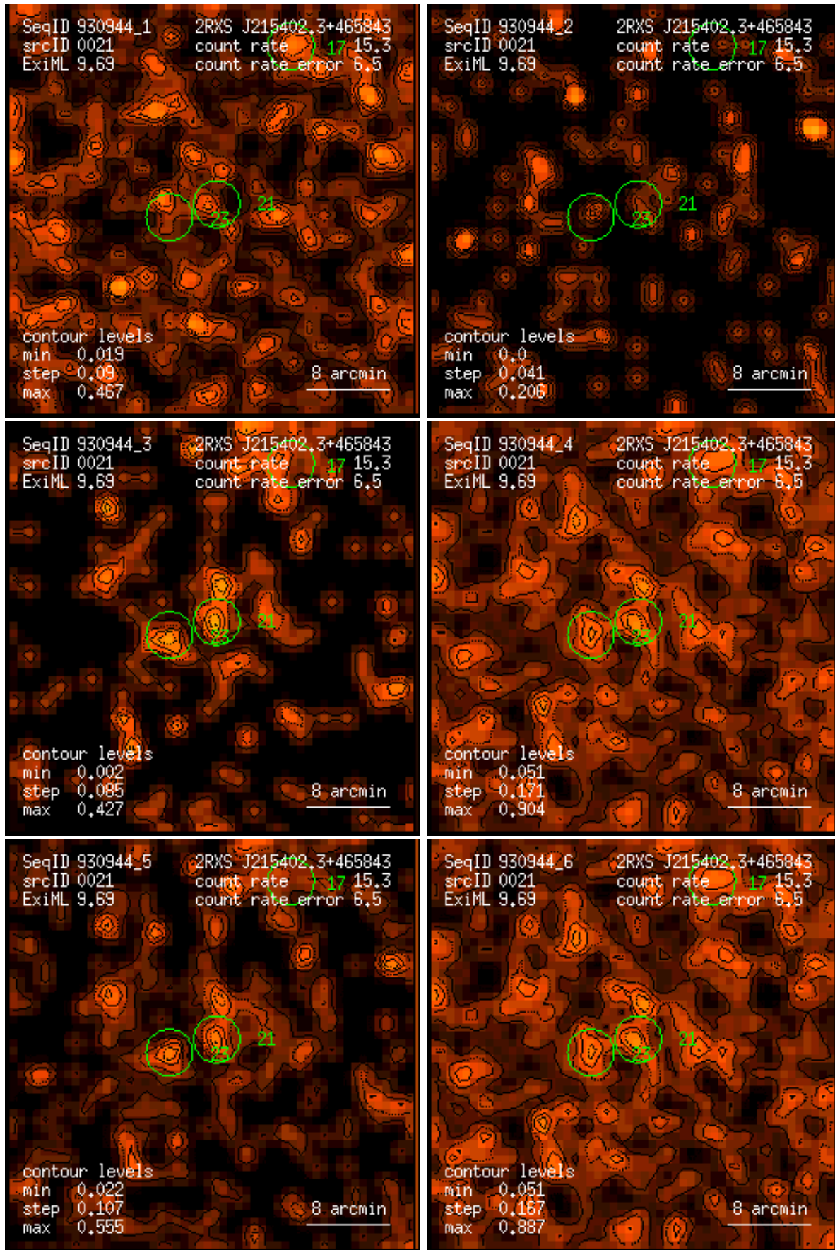
Figure 21: RASS 930944: detection 0021: band rate images, Gaussian filter: (1) PSPC channels 11 – 41, (2) 52 – 90, (3) 91 – 201, (4) 11 – 235, (5) 52 – 201, (6) 11 – 201. Broad band rates in counts/ks. Band rate contour levels in counts/ks/arcmin 2 .
