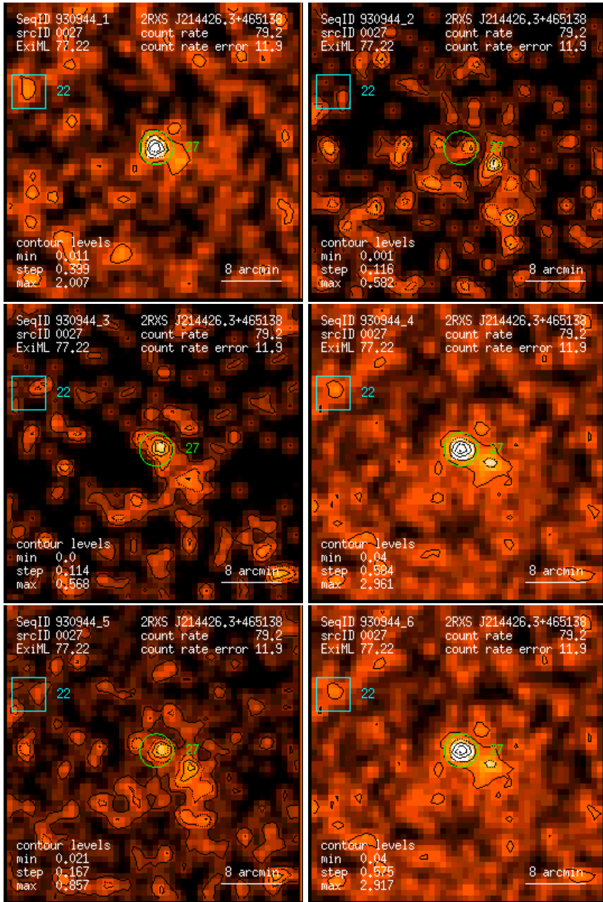
Figure 27: RASS 930944: detection 0027: band rate images, Gaussian filter: (1) PSPC channels 11 – 41, (2) 52 – 90, (3) 91 – 201, (4) 11 – 235, (5) 52 – 201, (6) 11 – 201. Broad band rates in counts/ks. Band rate contour levels in counts/ks/arcmin 2 .
