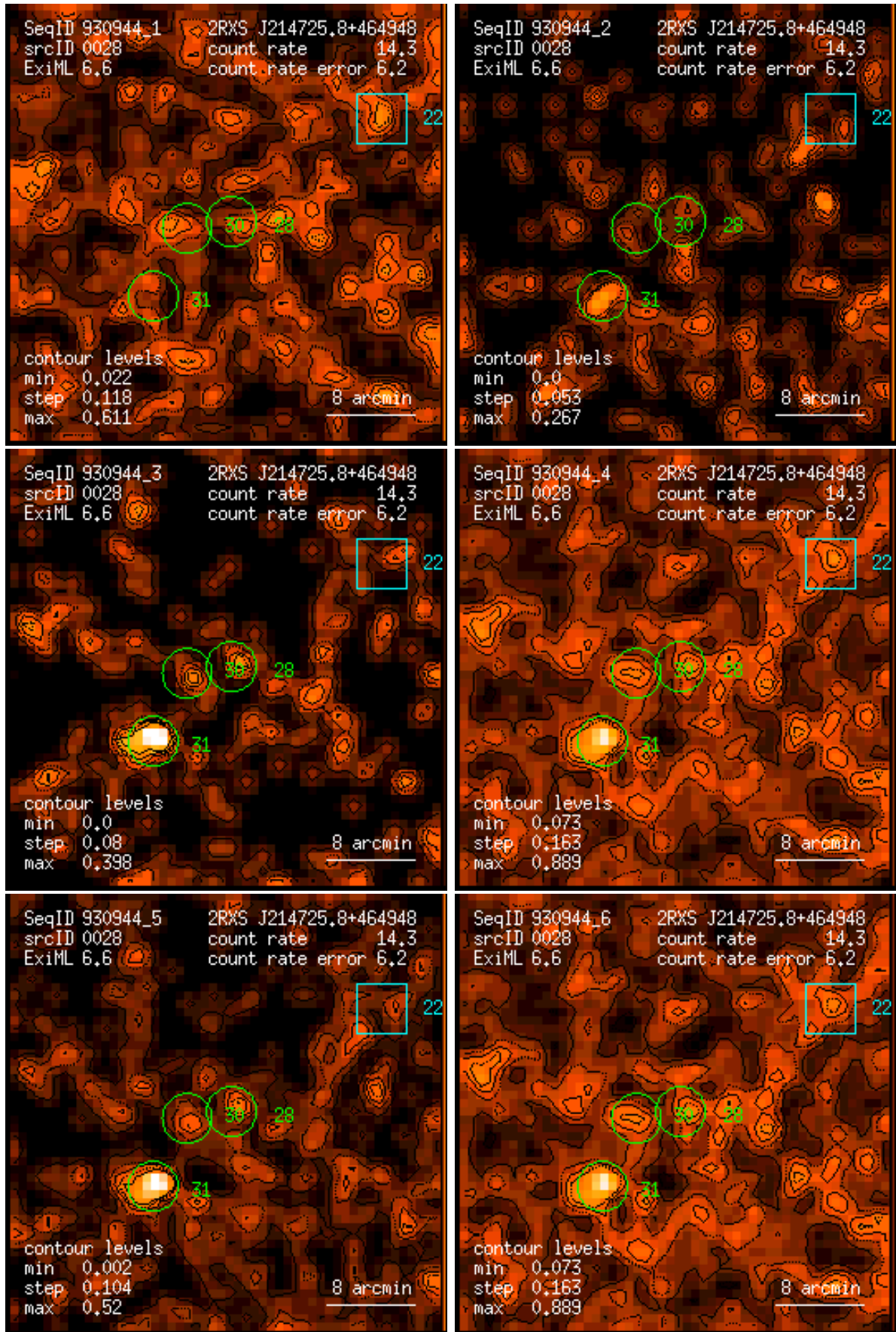
Figure 28: RASS 930944: detection 0028: band rate images, Gaussian filter: (1) PSPC channels 11 – 41, (2) 52 – 90, (3) 91 – 201, (4) 11 – 235, (5) 52 – 201, (6) 11 – 201. Broad band rates in counts/ks. Band rate contour levels in counts/ks/arcmin 2 .
