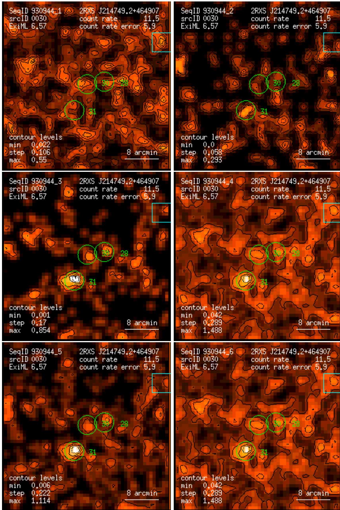
Figure 30: RASS 930944: detection 0030: band rate images, Gaussian filter: (1) PSPC channels 11 – 41, (2) 52 – 90, (3) 91 – 201, (4) 11 – 235, (5) 52 – 201, (6) 11 – 201. Broad band rates in counts/ks. Band rate contour levels in counts/ks/arcmin 2 .
