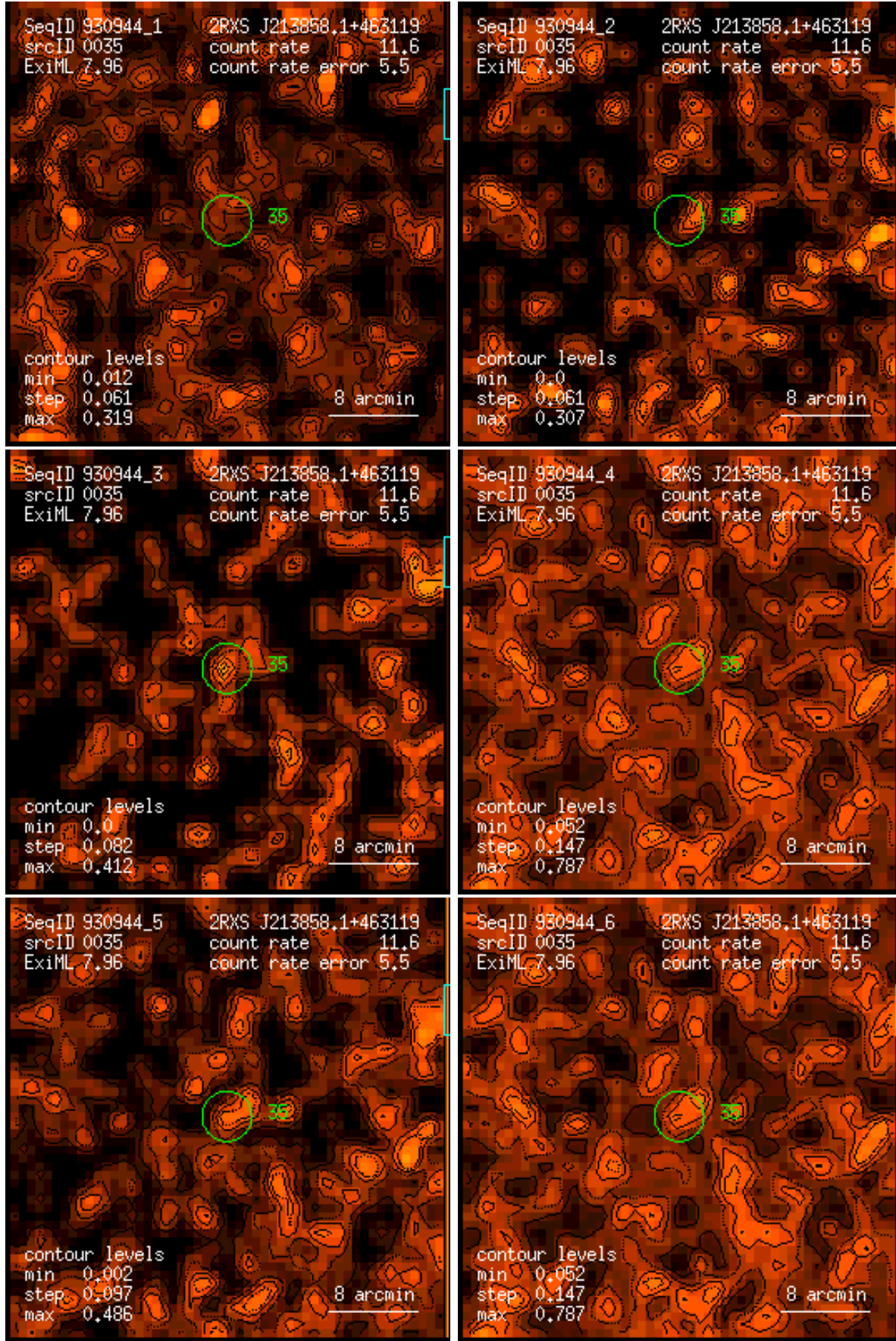
Figure 35: RASS 930944: detection 0035: band rate images, Gaussian filter: (1) PSPC channels 11 – 41, (2) 52 – 90, (3) 91 – 201, (4) 11 – 235, (5) 52 – 201, (6) 11 – 201. Broad band rates in counts/ks. Band rate contour levels in counts/ks/arcmin 2 .
