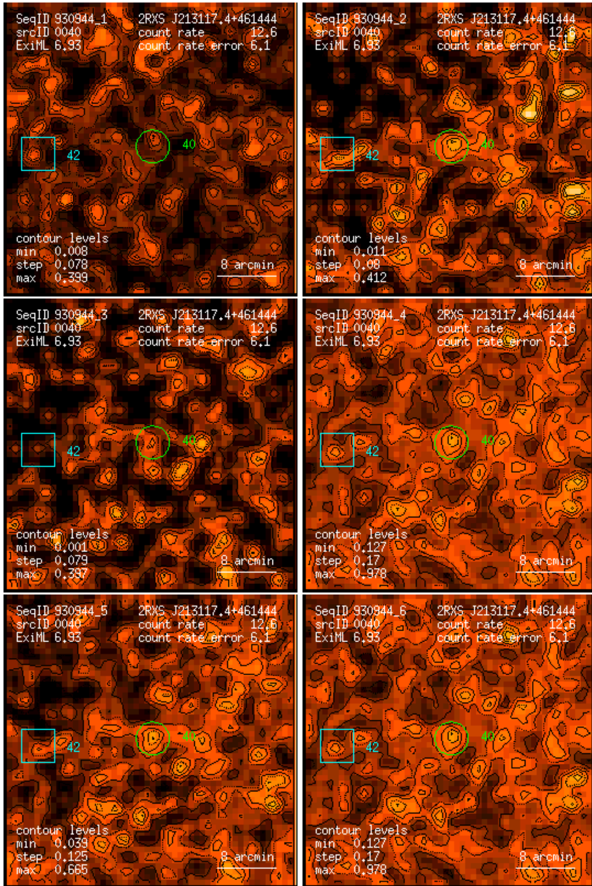
Figure 40: RASS 930944: detection 0040: band rate images, Gaussian filter: (1) PSPC channels 11 – 41, (2) 52 – 90, (3) 91 – 201, (4) 11 – 235, (5) 52 – 201, (6) 11 – 201. Broad band rates in counts/ks. Band rate contour levels in counts/ks/arcmin 2 .
