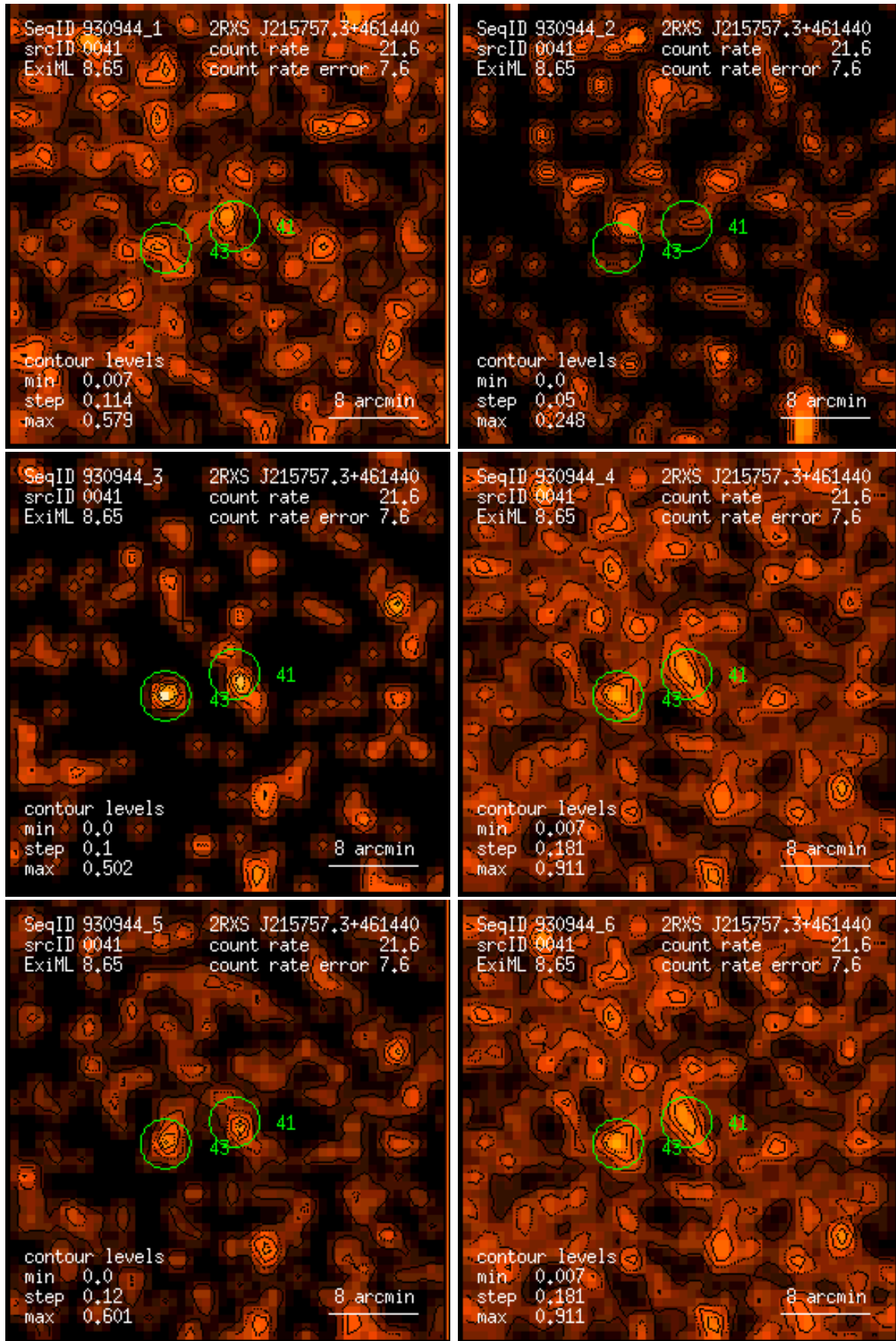
Figure 41: RASS 930944: detection 0041: band rate images, Gaussian filter: (1) PSPC channels 11 – 41, (2) 52 – 90, (3) 91 – 201, (4) 11 – 235, (5) 52 – 201, (6) 11 – 201. Broad band rates in counts/ks. Band rate contour levels in counts/ks/arcmin 2 .
