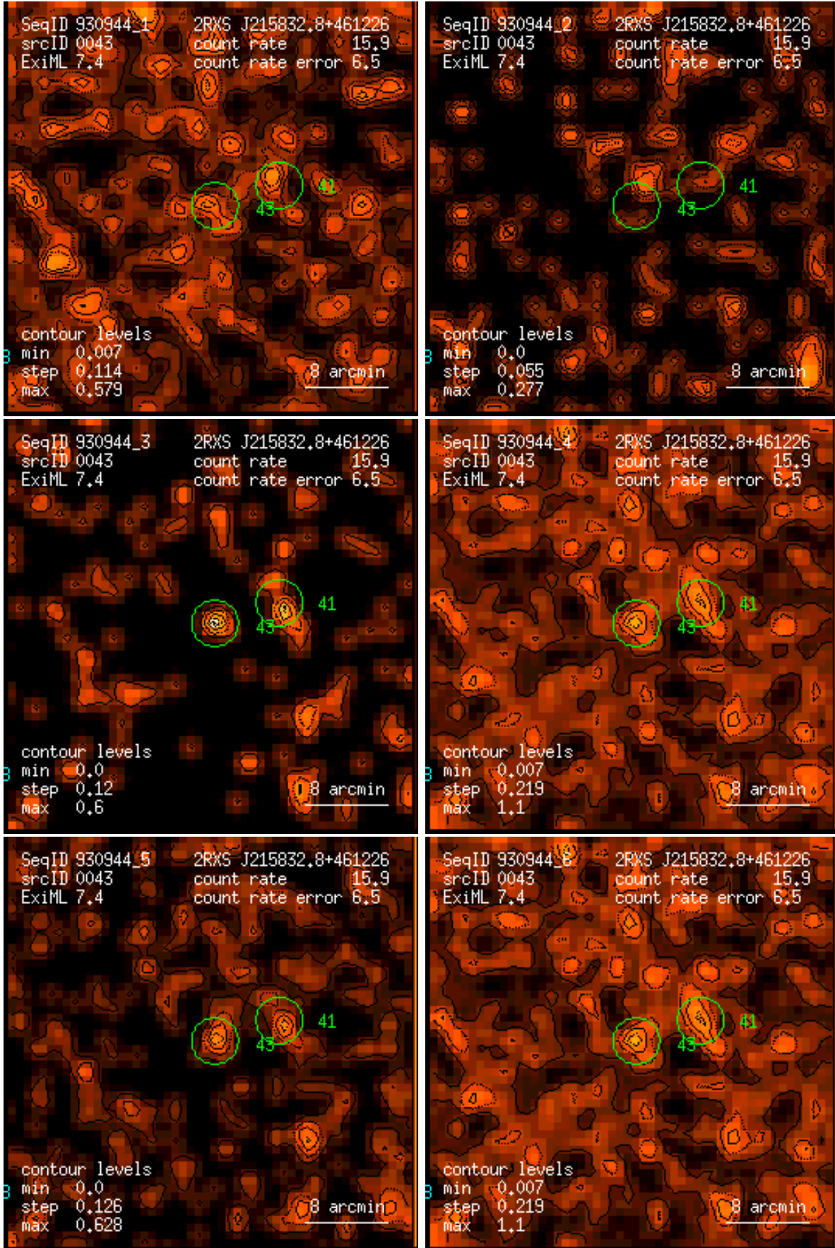
Figure 43: RASS 930944: detection 0043: band rate images, Gaussian filter: (1) PSPC channels 11 – 41, (2) 52 – 90, (3) 91 – 201, (4) 11 – 235, (5) 52 – 201, (6) 11 – 201. Broad band rates in counts/ks. Band rate contour levels in counts/ks/arcmin 2 .
