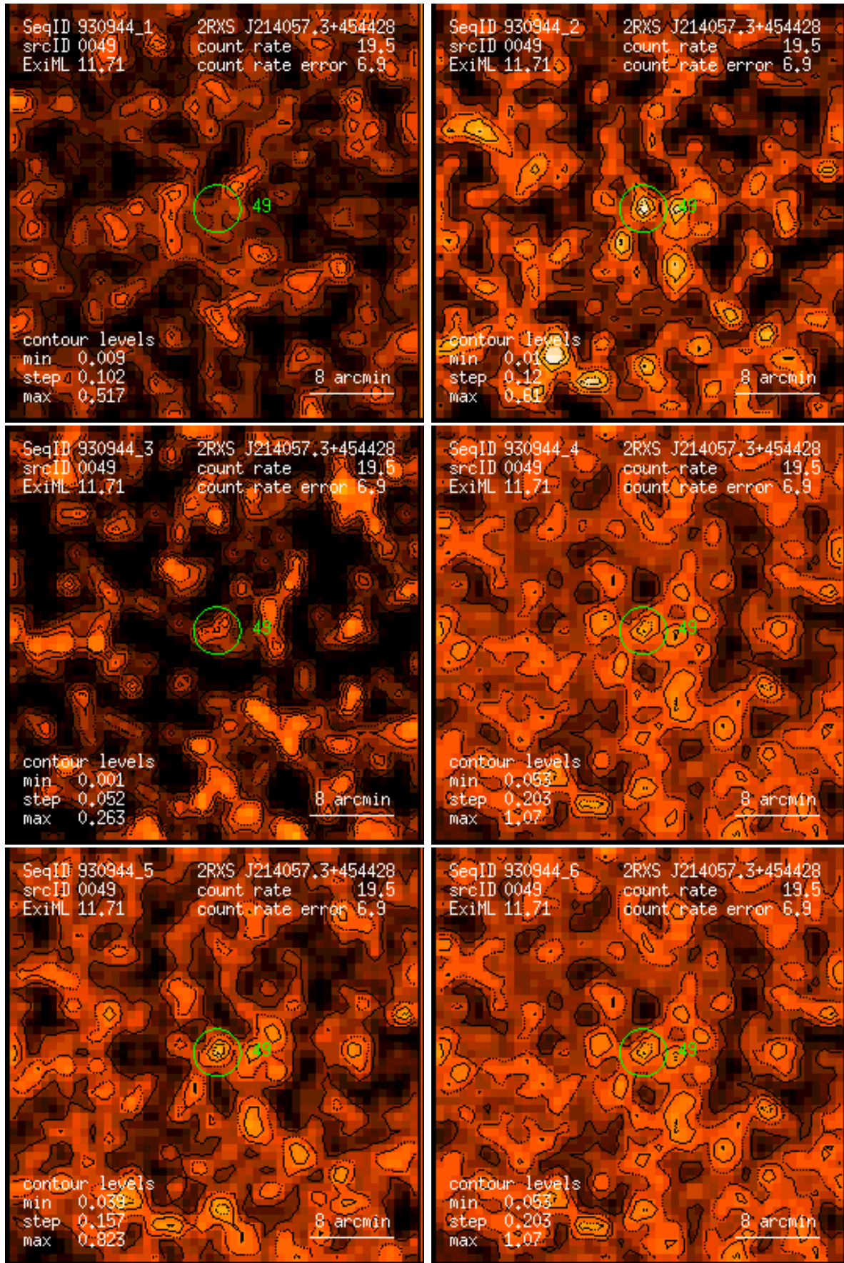
Figure 49: RASS 930944: detection 0049: band rate images, Gaussian filter: (1) PSPC channels 11 – 41, (2) 52 – 90, (3) 91 – 201, (4) 11 – 235, (5) 52 – 201, (6) 11 – 201. Broad band rates in counts/ks. Band rate contour levels in counts/ks/arcmin 2 .
