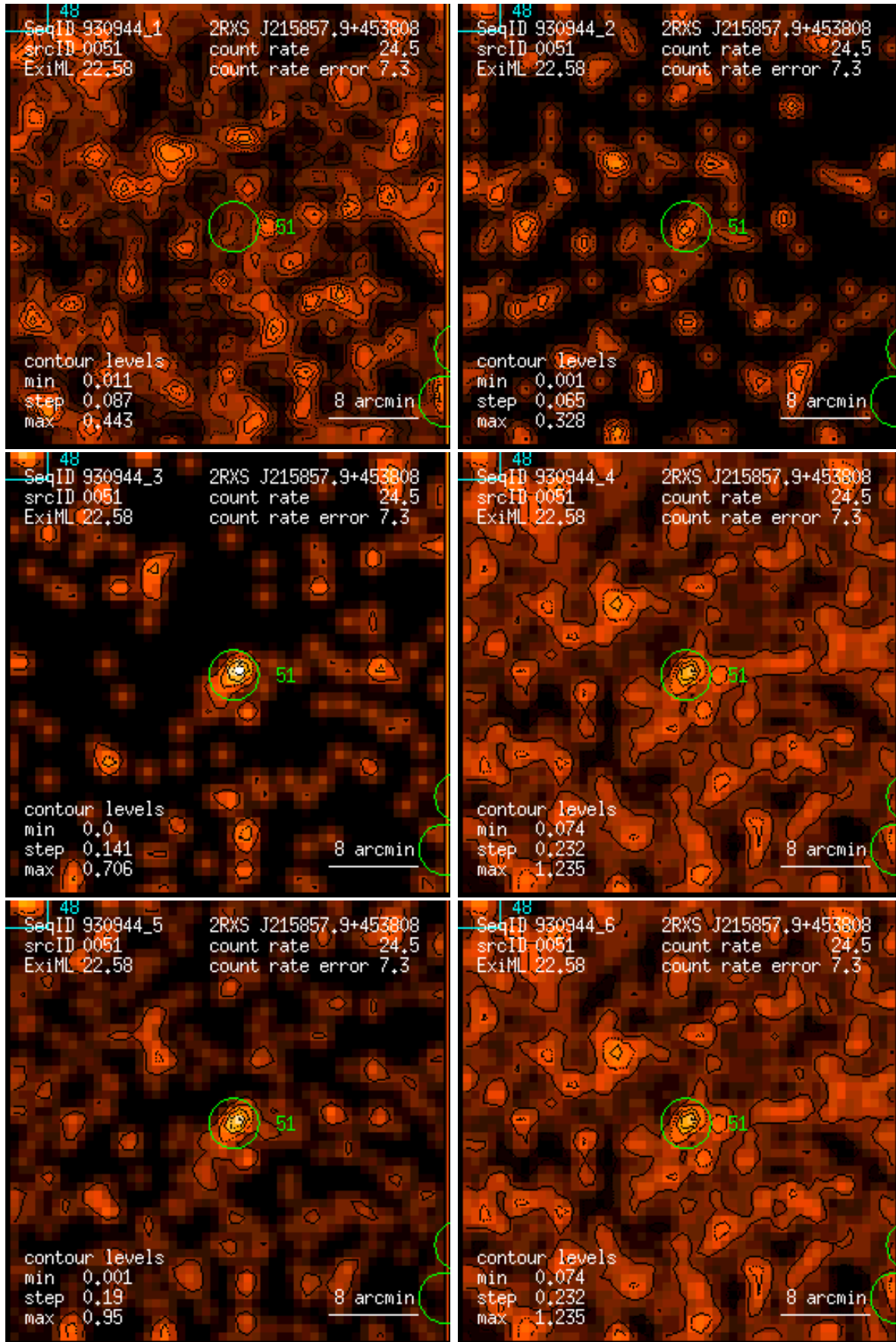
Figure 51: RASS 930944: detection 0051: band rate images, Gaussian filter: (1) PSPC channels 11 – 41, (2) 52 – 90, (3) 91 – 201, (4) 11 – 235, (5) 52 – 201, (6) 11 – 201. Broad band rates in counts/ks. Band rate contour levels in counts/ks/arcmin 2 .
