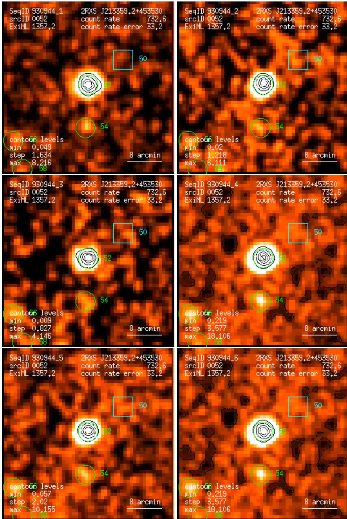
Figure 52: RASS 930944: detection 0052: band rate images, Gaussian filter: (1) PSPC channels 11 – 41, (2) 52 – 90, (3) 91 – 201, (4) 11 – 235, (5) 52 – 201, (6) 11 – 201. Broad band rates in counts/ks. Band rate contour levels in counts/ks/arcmin 2 .
