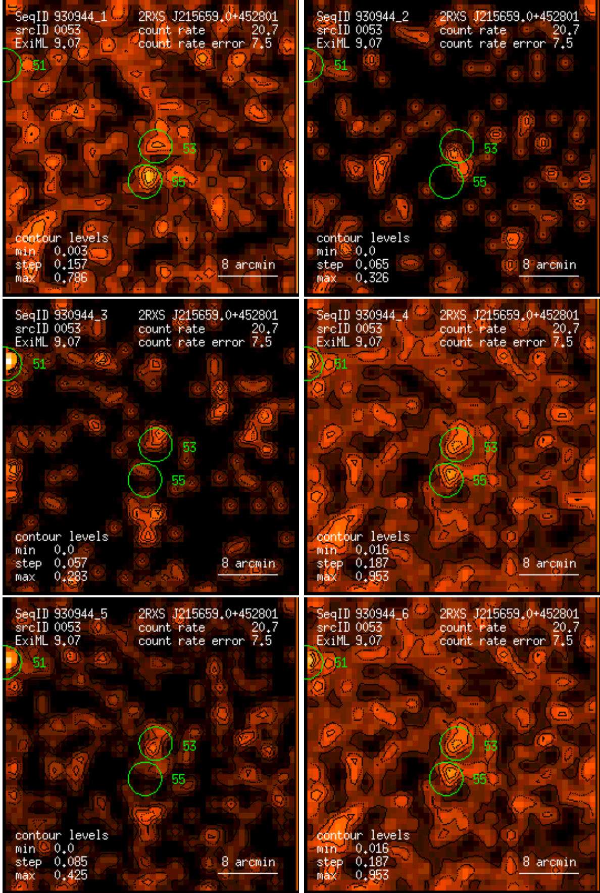
Figure 53: RASS 930944: detection 0053: band rate images, Gaussian filter: (1) PSPC channels 11 – 41, (2) 52 – 90, (3) 91 – 201, (4) 11 – 235, (5) 52 – 201, (6) 11 – 201. Broad band rates in counts/ks. Band rate contour levels in counts/ks/arcmin 2 .
