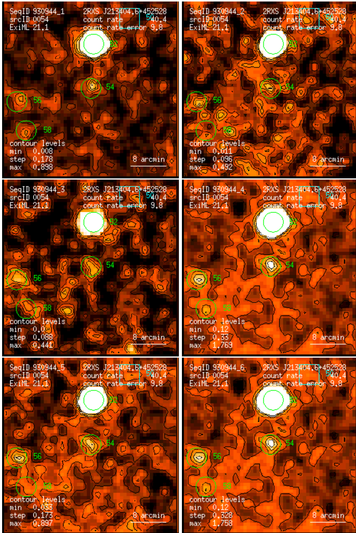
Figure 54: RASS 930944: detection 0054: band rate images, Gaussian filter: (1) PSPC channels 11 – 41, (2) 52 – 90, (3) 91 – 201, (4) 11 – 235, (5) 52 – 201, (6) 11 – 201. Broad band rates in counts/ks. Band rate contour levels in counts/ks/arcmin 2 .
