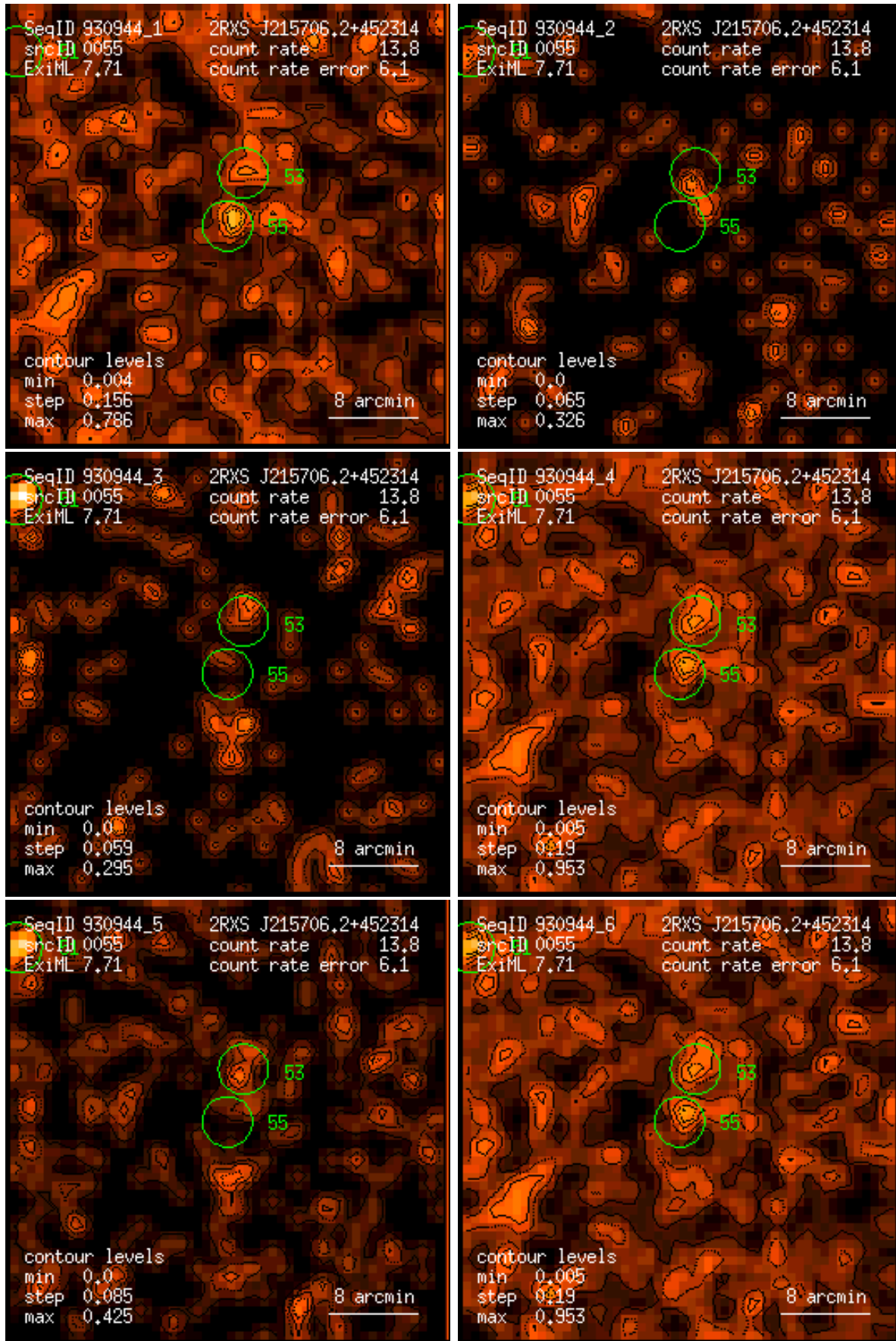
Figure 55: RASS 930944: detection 0055: band rate images, Gaussian filter: (1) PSPC channels 11 – 41, (2) 52 – 90, (3) 91 – 201, (4) 11 – 235, (5) 52 – 201, (6) 11 – 201. Broad band rates in counts/ks. Band rate contour levels in counts/ks/arcmin 2 .
