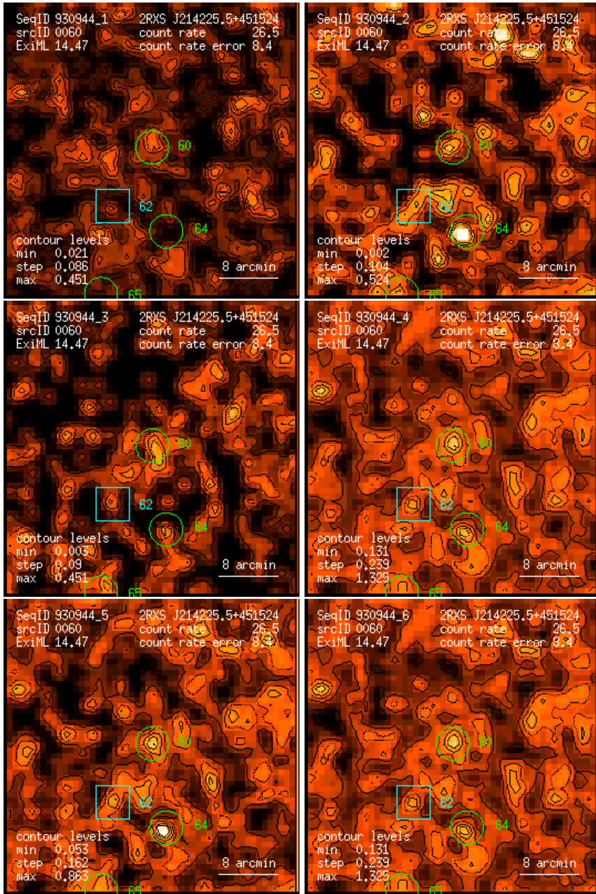
Figure 60: RASS 930944: detection 0060: band rate images, Gaussian filter: (1) PSPC channels 11 – 41, (2) 52 – 90, (3) 91 – 201, (4) 11 – 235, (5) 52 – 201, (6) 11 – 201. Broad band rates in counts/ks. Band rate contour levels in counts/ks/arcmin 2 .
