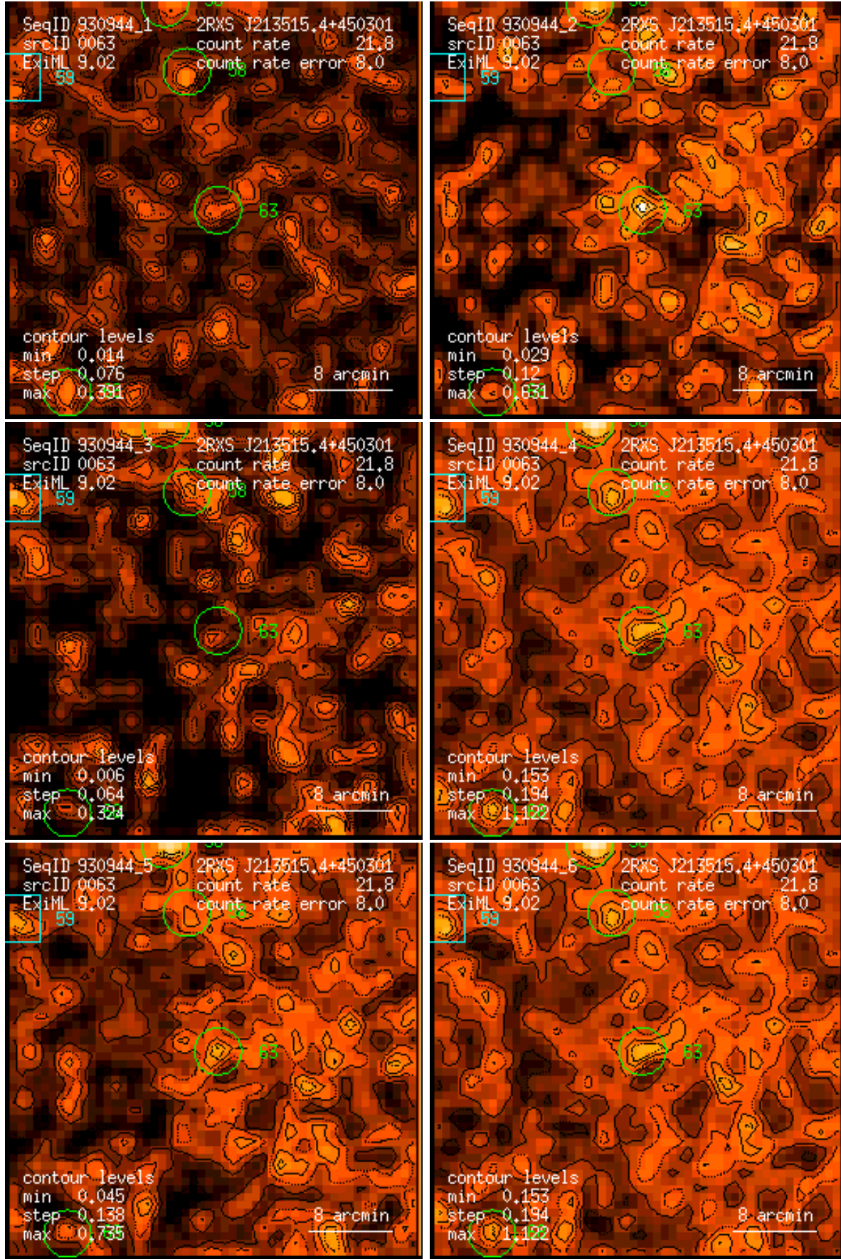
Figure 63: RASS 930944: detection 0063: band rate images, Gaussian filter: (1) PSPC channels 11 – 41, (2) 52 – 90, (3) 91 – 201, (4) 11 – 235, (5) 52 – 201, (6) 11 – 201. Broad band rates in counts/ks. Band rate contour levels in counts/ks/arcmin 2 .
